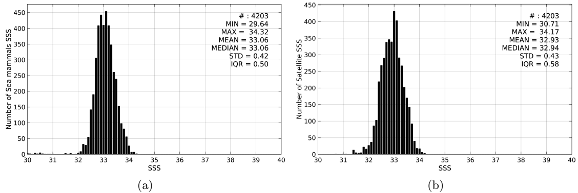
Figure 2: Histograms of SSS from Sea mammals (a) and SMOS-L3-CATDS-CPDC-V3-MONTHLY-25KM (b) considering all match-up pairs per bins of 0.1 over the North Pacific Ocean Pi-MEP region and for the full satellite product period.
