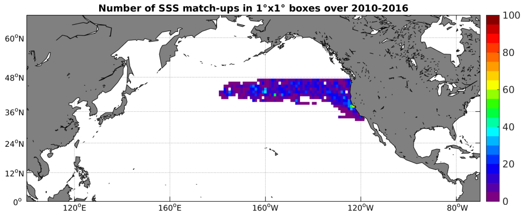
Figure 4: Number of SSS match-ups between Sea mammals SSS and the SMOS-L3-CATDS-CPDC-V3-MONTHLY-25KM SSS product for the North Pacific Ocean Pi-MEP region over 1^\circ \times 1^\circ boxes and for the full satellite product period.
