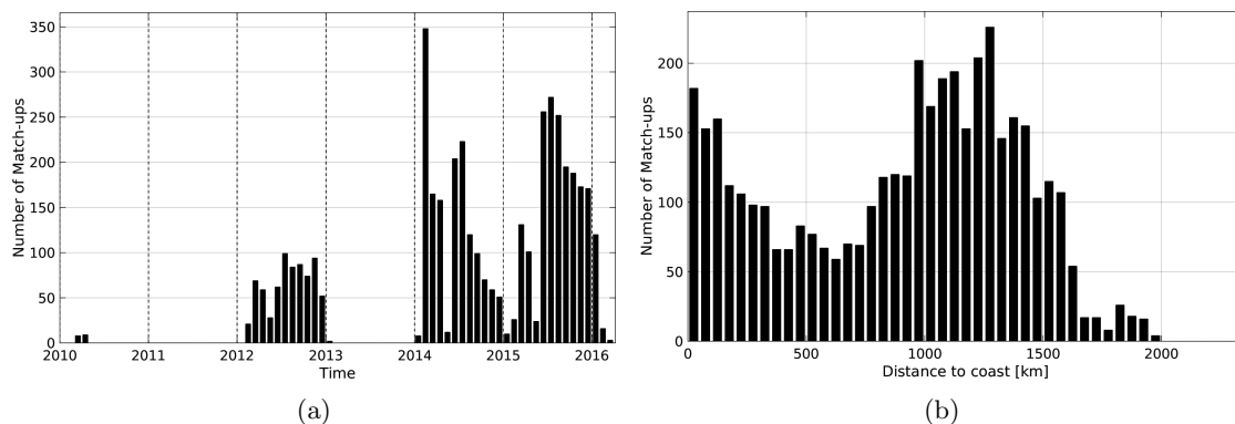
Figure 1: Number of match-ups between Sea mammals and SMOS-L3-CATDS-CPDC-V3-MONTHLY-25KM SSS as a function of time (a) and as function of the distance to coast (b) over the North Pacific Ocean Pi-MEP region and for the full satellite product period.
