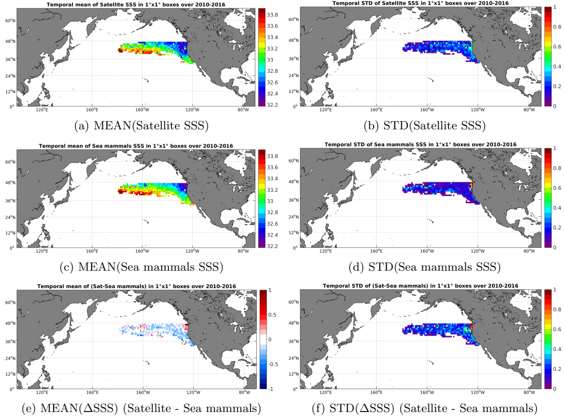
Figure 6: Temporal mean (left) and STD (right) of SSS from SMOS-L3-CATDS-CPDC-V3-MONTHLY-25KM (top), Sea mammals (middle), and of \Delta SSS (Satellite - Sea mammals). Only match-up pairs are used to generate these maps.
