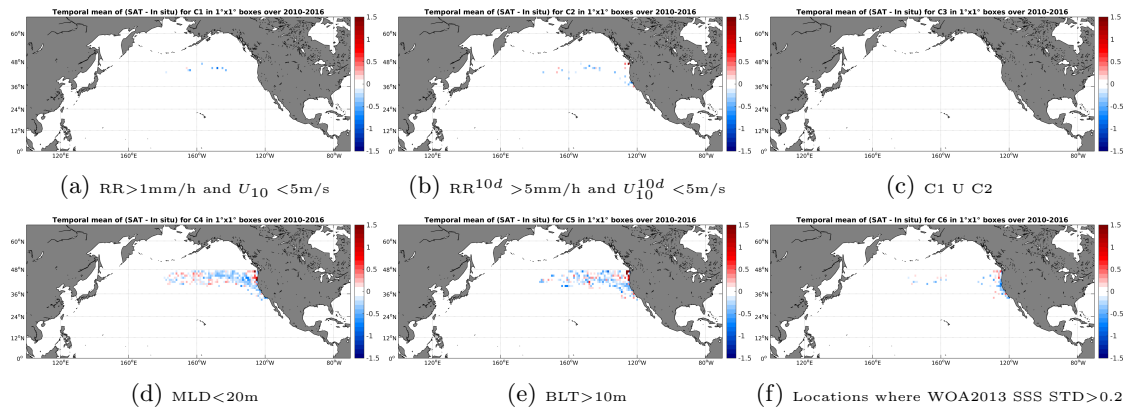
Figure 12: Temporal mean gridded over spatial boxes of size 1^\circ \times 1^\circ of \Delta SSS (SMOS-L3-CATDS-CPDC-V3-MONTHLY-25KM - Sea mammals) for 6 different subdatasets corresponding to: RR > 1\text{mm/h} and U_{10} < 5\text{m/s} (a), RR^{10d} > 5\text{mm/h} and U_{10}^{10d} < 5\text{m/s} (b), C1 U C2 (c), MLD < 20\text{m} (d), BLT > 10\text{m} (e), Locations where WOA2013 SSS STD > 0.2 (f).
