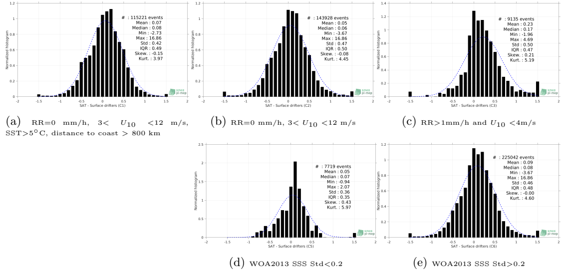
Figure 12: Normalized histogram of \Delta SSS (SMOS-L3-CATDS-CPDC-V3-MONTHLY-25KM - Surface drifters) for 5 different subdatasets corresponding to: RR=0 mm/h, 3 < U_{10} < 12 m/s, SST > 5°C, distance to coast > 800 km (a), RR=0 mm/h, 3 < U_{10} < 12 m/s (b), RR > 1mm/h and U_{10} < 4 m/s (c), WOA2013 SSS Std < 0.2 (d), WOA2013 SSS Std > 0.2 (e).
