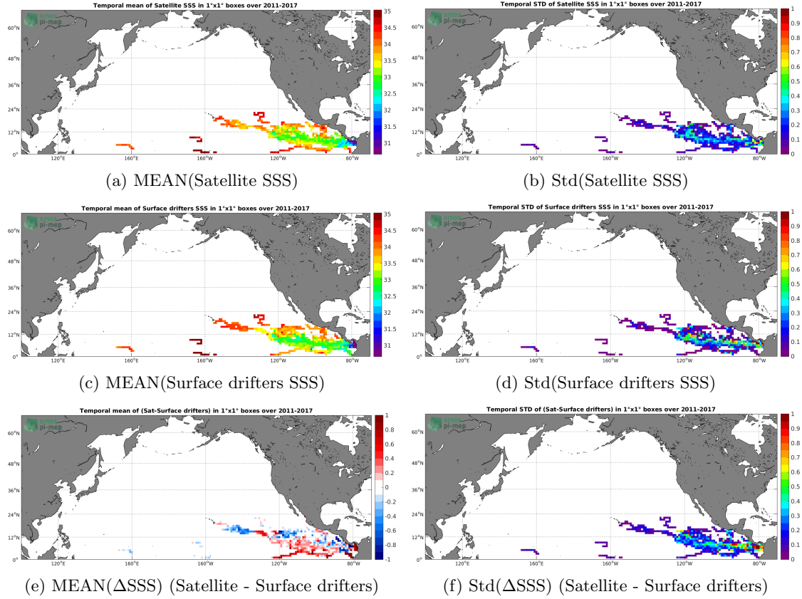
Figure 5: Temporal mean (left) and Std (right) of SSS from SMOS-L3-CATDS-CPDC-V3-MONTHLY-25KM (top), Surface drifters (middle), and of \Delta SSS (Satellite - Surface drifters). Only match-up pairs are used to generate these maps.
