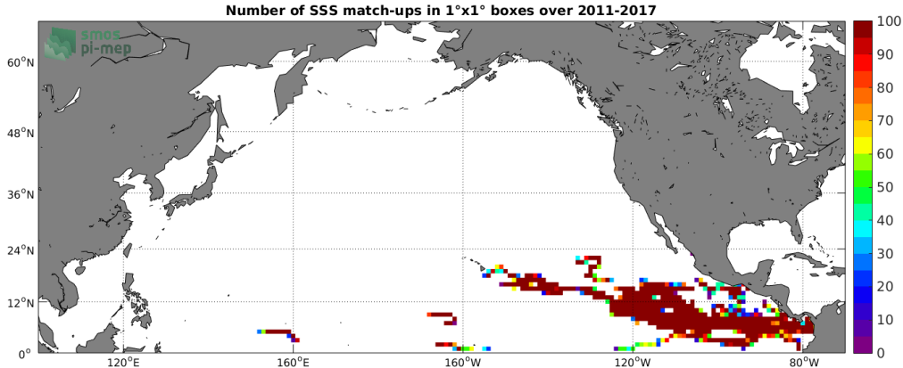
Figure 3: Number of SSS match-ups between Surface drifters SSS and the SMOS-L3-CATDS-CPDC-V3-MONTHLY-25KM SSS product for the North Pacific Ocean Pi-MEP region over 1°x1° boxes and for the full satellite product period.
