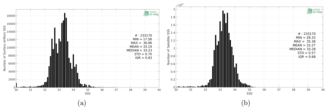
Figure 2: Histograms of SSS from Surface drifters (a) and SMOS-L3-CATDS-CPDC-V3-MONTHLY-25KM (b) considering all match-up pairs per bins of 0.1 over the North Pacific Ocean Pi-MEP region and for the full satellite product period.
