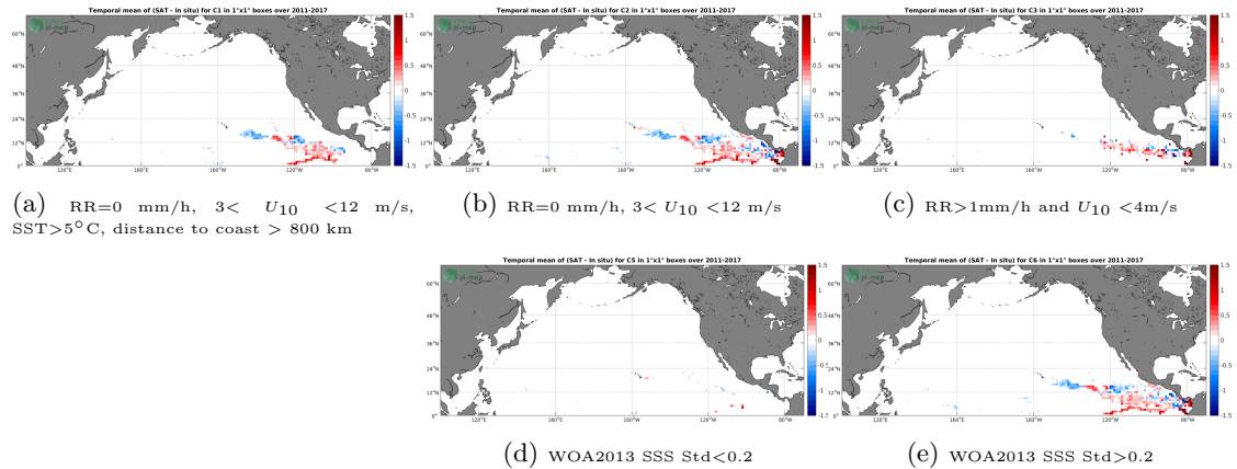
Figure 11: Temporal mean gridded over spatial boxes of size 1^\circ \times 1^\circ of \Delta SSS (SMOS-L3-CATDS-CPDC-V3-MONTHLY-25KM - Surface drifters) for 5 different subdatasets corresponding to:RR=0 mm/h, 3 < U_{10} < 12 m/s, SST >5^\circ C, distance to coast > 800 km (a), RR=0 mm/h, 3 < U_{10} < 12 m/s (b), RR >1 mm/h and U_{10} < 4 m/s (c), WOA2013 SSS Std <0.2 (d), WOA2013 SSS Std >0.2 (e).
