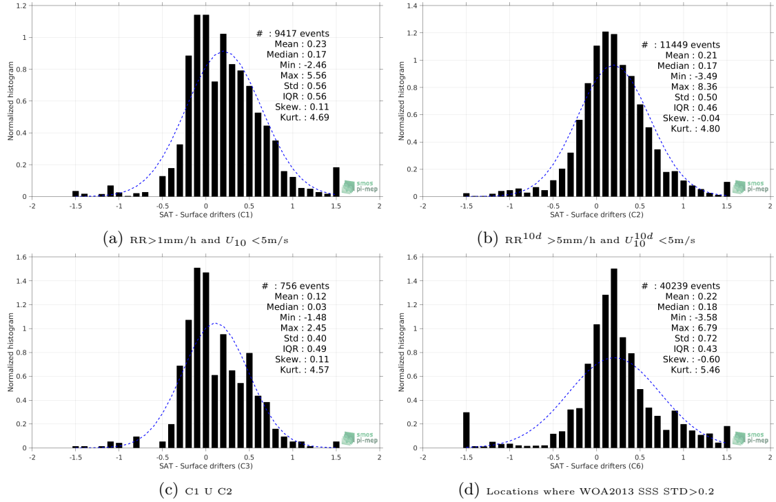
Figure 12: Normalized histogram of \Delta SSS (SMOS-L3-CATDS-CPDC-V3-MONTHLY-25KM - Surface drifters) for 6 different subdatasets corresponding to: RR > 1mm/h and U_{10} < 5 m/s (a), RR^{10d} > 5 mm/h and U_{10}^{10d} < 5 m/s (b), C1 U C2 (c), Locations where WOA2013 SSS STD > 0.2 (d).
