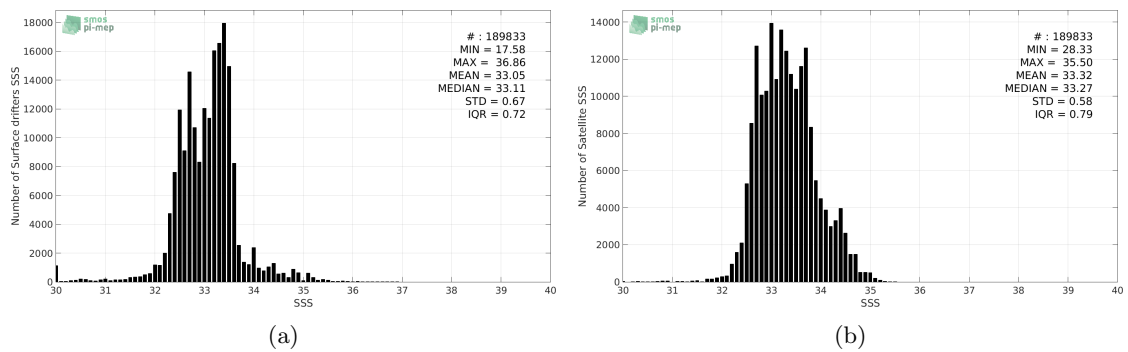
Figure 2: Histograms of SSS from Surface drifters (a) and SMOS-L3-CATDS-CPDC-V3-MONTHLY-25KM (b) considering all match-up pairs per bins of 0.1 over the North Pacific Ocean Pi-MEP region and for the full satellite product period.
