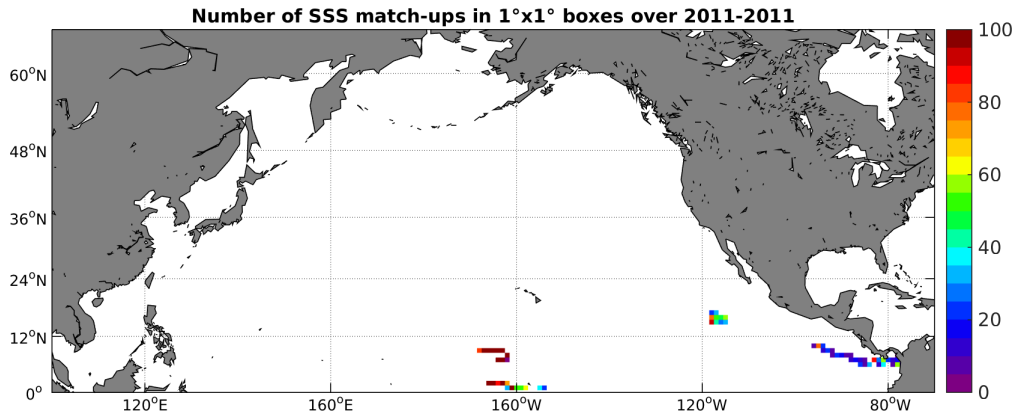
Figure 3: Number of SSS match-ups between Surface drifters SSS and the SMOS-L3-CATDS-CPDC-V3-MONTHLY-25KM SSS product for the North Pacific Ocean Pi-MEP region over 1^\circ \times 1^\circ boxes and for the full satellite product period.
