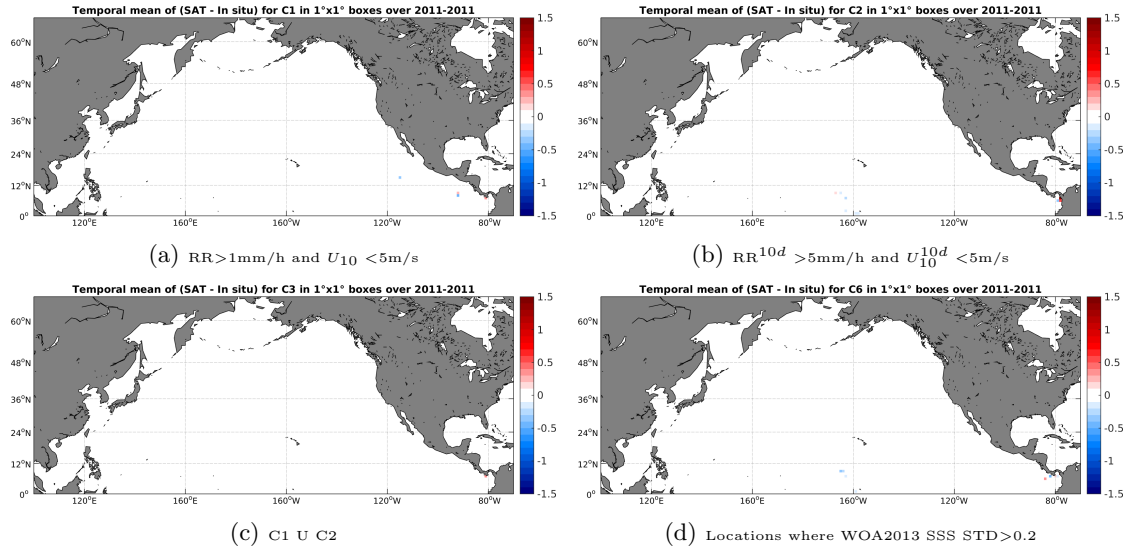
Figure 11: Temporal mean gridded over spatial boxes of size 1^\circ \times 1^\circ of \Delta SSS (SMOS-L3-CATDS-CPDC-V3-MONTHLY-25KM - Surface drifters) for 4 different subdatasets corresponding to: RR > 1\text{mm/h} and U_{10} < 5\text{m/s} (a), RR^{10d} > 5\text{mm/h} and U_{10}^{10d} < 5\text{m/s} (b), C1 U C2 (c), Locations where WOA2013 SSS STD > 0.2 (d).
