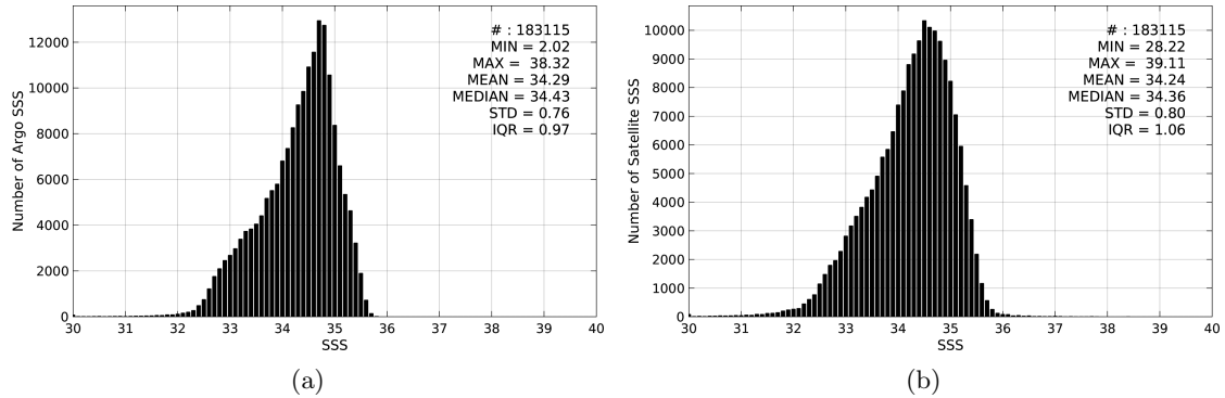
Figure 2: Histograms of SSS from Argo (a) and SMOS-L3-CATDS-CPDC-V3-MONTHLY-25KM (b) considering all match-up pairs per bins of 0.1 over the North Pacific Ocean Pi-MEP region and for the full satellite product period.
