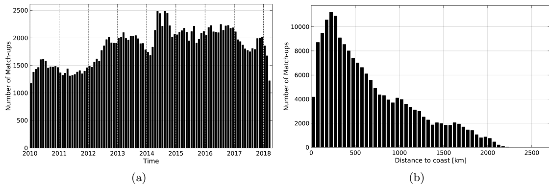
Figure 1: Number of match-ups between Argo and SMOS-L3-CATDS-CPDC-V3-MONTHLY-25KM SSS as a function of time (a) and as function of the distance to coast (b) over the North Pacific Ocean Pi-MEP region and for the full satellite product period.
