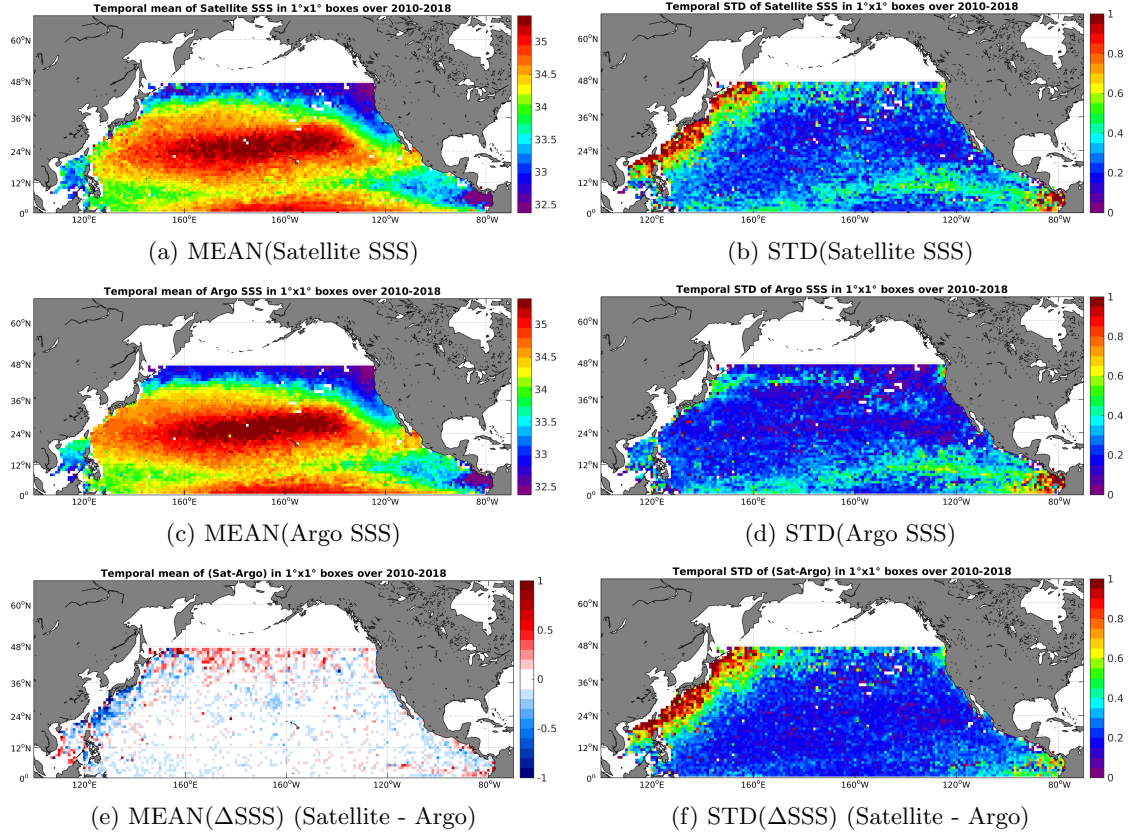
Figure 6: Temporal mean (left) and STD (right) of SSS from SMOS-L3-CATDS-CPDC-V3-MONTHLY-25KM (top), Argo (middle), and of \Delta\text{SSS} (Satellite - Argo). Only match-up pairs are used to generate these maps.
