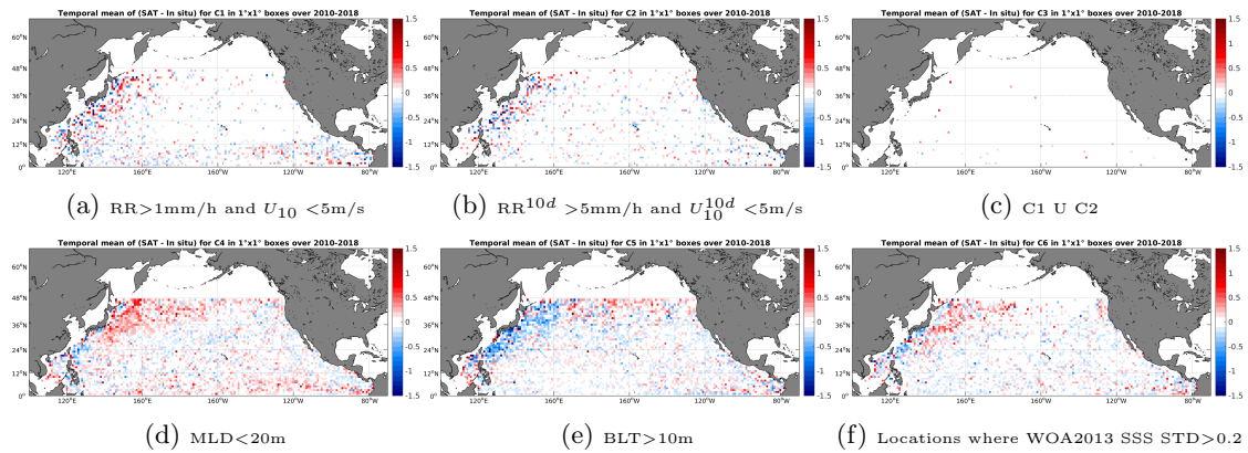
Figure 12: Temporal mean gridded over spatial boxes of size 1^\circ \times 1^\circ of \Delta SSS (SMOS-L3-CATDS-CPDC-V3-MONTHLY-25KM - Argo) for 6 different subdatasets corresponding to: RR > 1\text{mm/h} and U_{10} < 5\text{m/s} (a), RR^{10d} > 5\text{mm/h} and U_{10}^{10d} < 5\text{m/s} (b), C1 U C2 (c), MLD < 20\text{m} (d), BLT > 10\text{m} (e), Locations where WOA2013 SSS STD > 0.2 (f).
