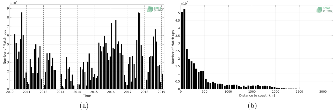
Figure 1: Number of match-ups between TSG-SAMOS and SMOS-L3-CATDS-CPDC-V3-10DAYS-25KM SSS as a function of time (a) and as function of the distance to coast (b) over the North Pacific Ocean Pi-MEP region and for the full satellite product period.
