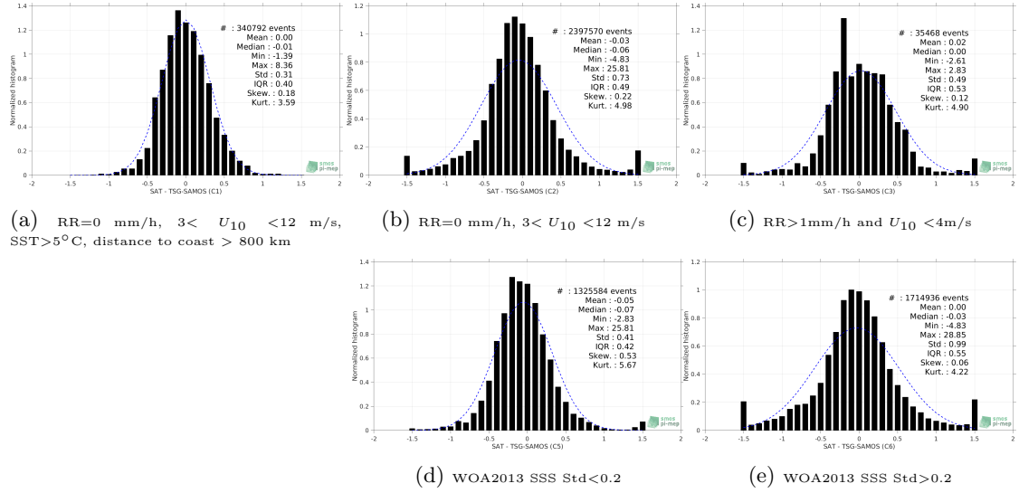
Figure 13: Normalized histogram of \Delta\text{SSS} (SMOS-L3-CATDS-CPDC-V3-10DAYS-25KM - TSG-SAMOS) for 5 different subdatasets corresponding to: RR=0 mm/h, 3 < U_{10} < 12 m/s, SST > 5^\circ\text{C} , distance to coast > 800 km (a), RR=0 mm/h, 3 < U_{10} < 12 m/s (b), RR > 1 mm/h and U_{10} < 4 m/s (c), WOA2013 SSS Std < 0.2 (d), WOA2013 SSS Std > 0.2 (e).
