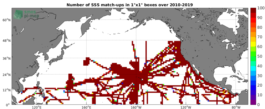
Figure 4: Number of SSS match-ups between TSG-SAMOS SSS and the SMOS-L3-CATDS-CPDC-V3-10DAYS-25KM SSS product for the North Pacific Ocean Pi-MEP region over 1^\circ \times 1^\circ boxes and for the full satellite product period.
