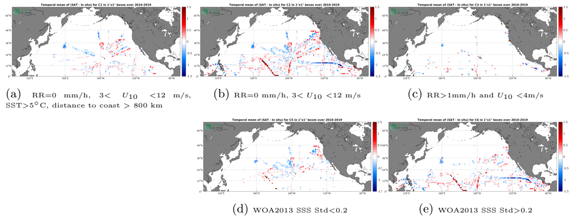
Figure 12: Temporal mean gridded over spatial boxes of size 1^\circ \times 1^\circ of \Delta SSS (SMOS-L3-CATDS-CPDC-V3-10DAYS-25KM - TSG-SAMOS) for 5 different subdatasets corresponding to:RR=0 mm/h, 3 < U_{10} < 12 m/s, SST >5^\circ C, distance to coast > 800 km (a), RR=0 mm/h, 3 < U_{10} < 12 m/s (b), RR >1 mm/h and U_{10} < 4 m/s (c), WOA2013 SSS Std <0.2 (d), WOA2013 SSS Std >0.2 (e).
