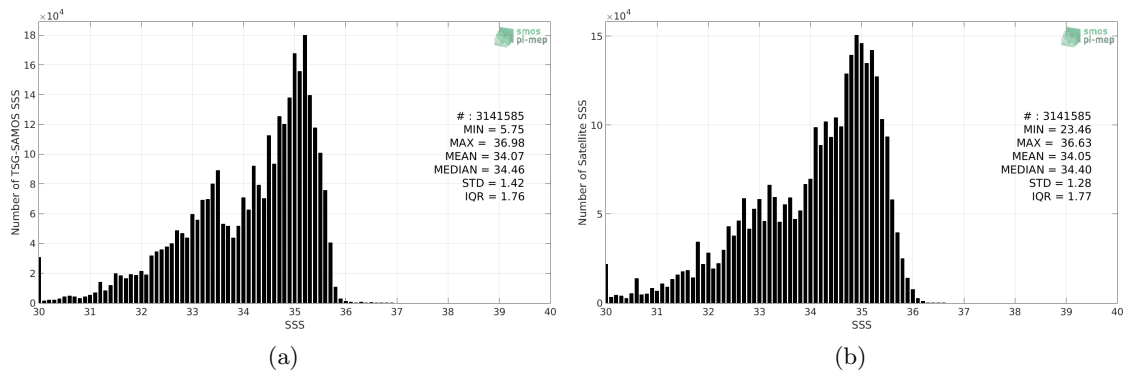
Figure 2: Histograms of SSS from TSG-SAMOS (a) and SMOS-L3-CATDS-CPDC-V3-10DAYS-25KM (b) considering all match-up pairs per bins of 0.1 over the North Pacific Ocean Pi-MEP region and for the full satellite product period.
