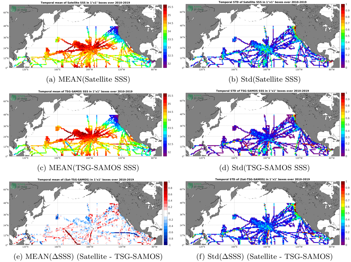
Figure 6: Temporal mean (left) and Std (right) of SSS from SMOS-L3-CATDS-CPDC-V3-10DAYS-25KM (top), TSG-SAMOS (middle), and of \Delta SSS (Satellite - TSG-SAMOS). Only match-up pairs are used to generate these maps.
