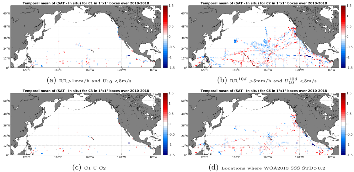
Figure 12: Temporal mean gridded over spatial boxes of size 1^\circ \times 1^\circ of \Delta SSS (SMOS-L3-CATDS-CPDC-V3-10DAYS-25KM - TSG-SAMOS) for 4 different subdatasets corresponding to:RR >1 mm/h and U_{10} < 5 m/s (a), RR^{10d} > 5 mm/h and U_{10}^{10d} < 5 m/s (b), C1 U C2 (c),Locations where WOA2013 SSS STD >0.2 (d).
