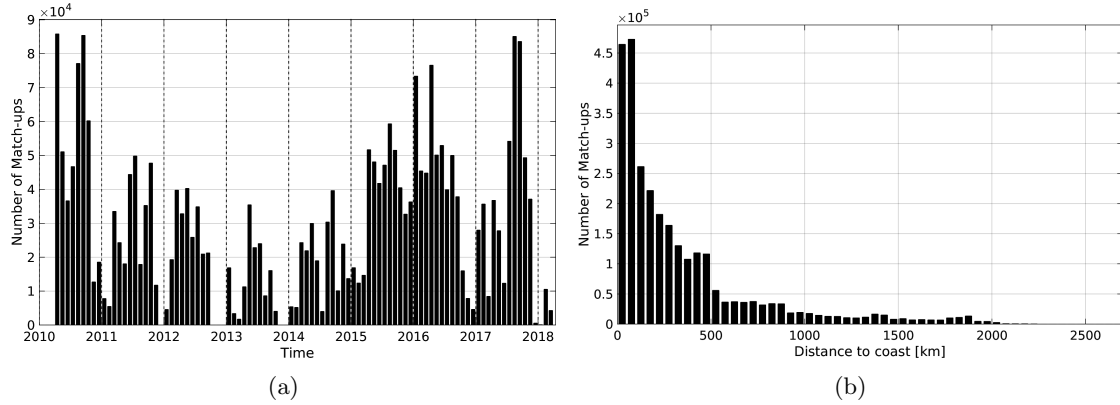
Figure 1: Number of match-ups between TSG-SAMOS and SMOS-L3-CATDS-CPDC-V3-10DAYS-25KM SSS as a function of time (a) and as function of the distance to coast (b) over the North Pacific Ocean Pi-MEP region and for the full satellite product period.
