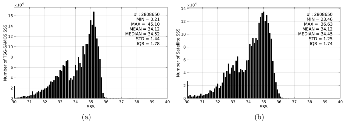
Figure 2: Histograms of SSS from TSG-SAMOS (a) and SMOS-L3-CATDS-CPDC-V3-10DAYS-25KM (b) considering all match-up pairs per bins of 0.1 over the North Pacific Ocean Pi-MEP region and for the full satellite product period.
