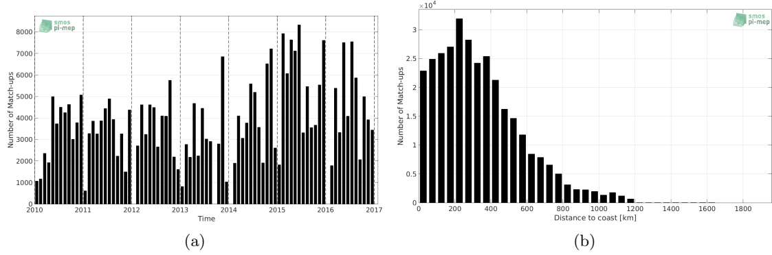
Figure 1: Number of match-ups between TSG-LEGOS-DM and SMOS-L3-CATDS-CPDC-V3-10DAYS-25KM SSS as a function of time (a) and as function of the distance to coast (b) over the North Pacific Ocean Pi-MEP region and for the full satellite product period.
