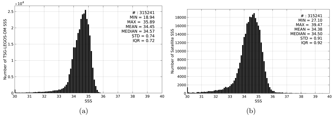
Figure 2: Histograms of SSS from TSG-LEGOS-DM (a) and SMOS-L3-CATDS-CPDC-V3-10DAYS-25KM (b) considering all match-up pairs per bins of 0.1 over the North Pacific Ocean Pi-MEP region and for the full satellite product period.
