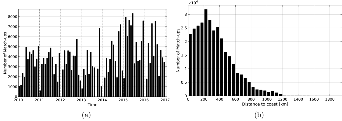
Figure 1: Number of match-ups between TSG-LEGOS-DM and SMOS-L3-CATDS-CPDC-V3-10DAYS-25KM SSS as a function of time (a) and as function of the distance to coast (b) over the North Pacific Ocean Pi-MEP region and for the full satellite product period.
