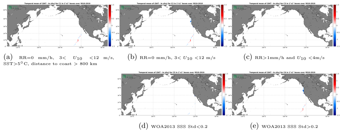
Figure 12: Temporal mean gridded over spatial boxes of size 1^\circ \times 1^\circ of \Delta SSS (SMOS-L3-CATDS-CPDC-V3-10DAYS-25KM - TSG-GOSUD-Sailing-ship) for 5 different subdatasets corresponding to:RR=0 mm/h, 3 < U_{10} < 12 m/s, SST >5^\circ C, distance to coast > 800 km (a), RR=0 mm/h, 3 < U_{10} < 12 m/s (b), RR >1 mm/h and U_{10} < 4 m/s (c), WOA2013 SSS Std <0.2 (d), WOA2013 SSS Std >0.2 (e).
