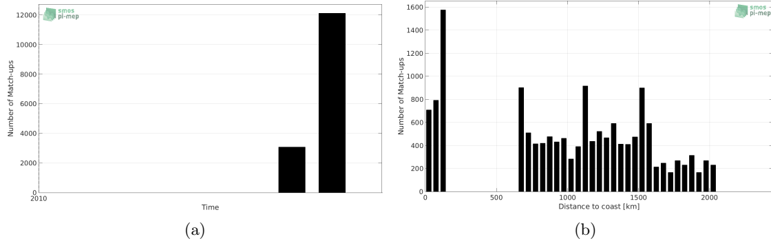
Figure 1: Number of match-ups between TSG-GOSUD-Sailing-ship and SMOS-L3-CATDS-CPDC-V3-10DAYS-25KM SSS as a function of time (a) and as function of the distance to coast (b) over the North Pacific Ocean Pi-MEP region and for the full satellite product period.
