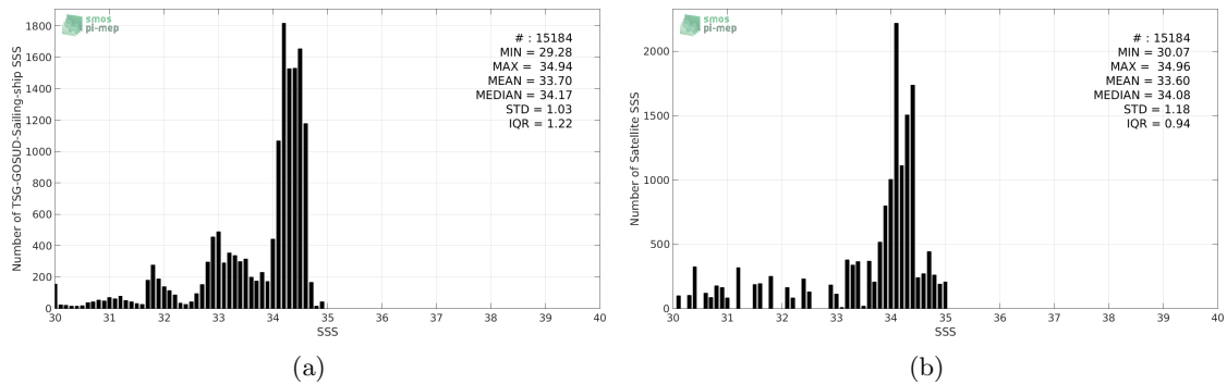
Figure 2: Histograms of SSS from TSG-GOSUD-Sailing-ship (a) and SMOS-L3-CATDS-CPDC-V3-10DAYS-25KM (b) considering all match-up pairs per bins of 0.1 over the North Pacific Ocean Pi-MEP region and for the full satellite product period.
