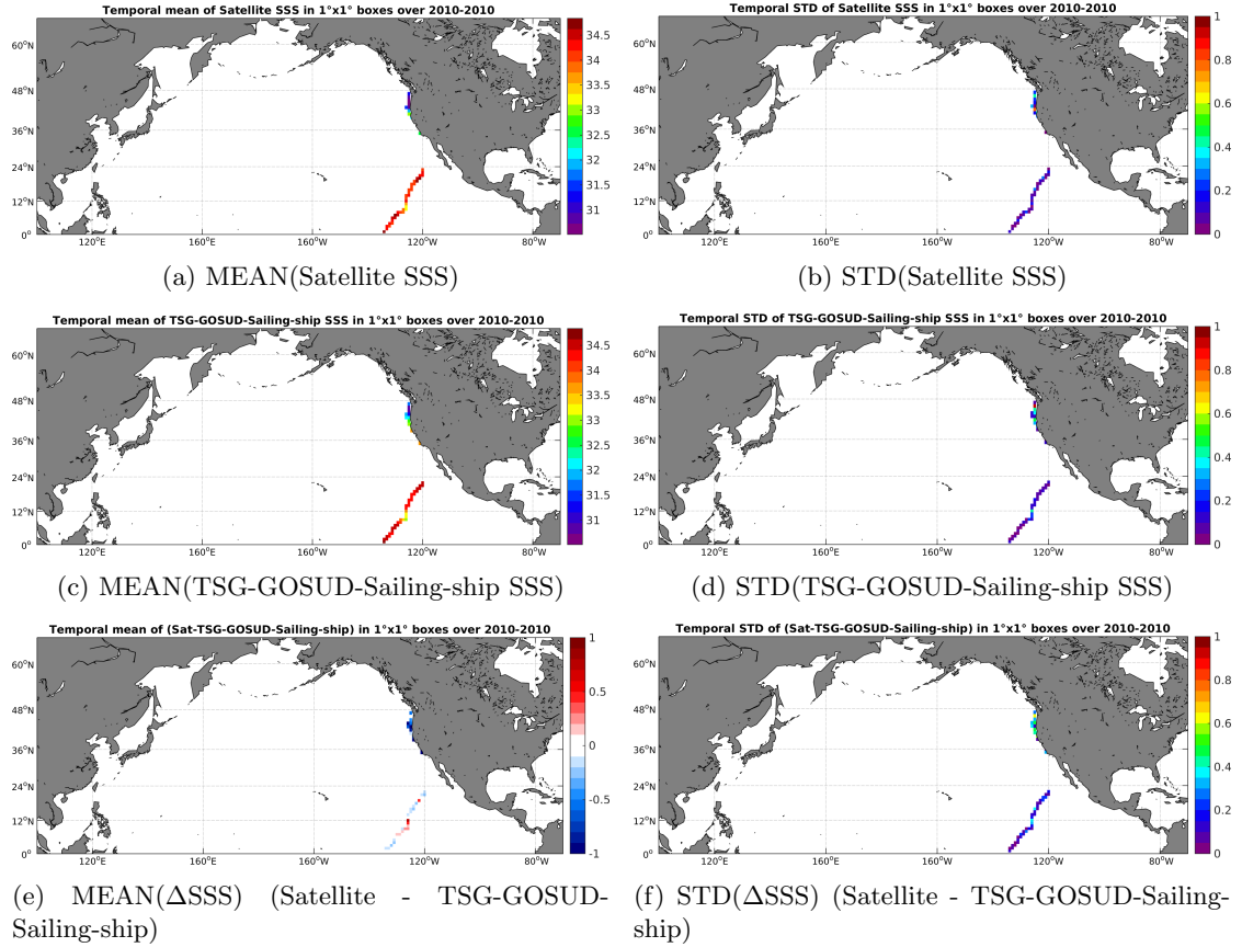
Figure 6: Temporal mean (left) and STD (right) of SSS from SMOS-L3-CATDS-CPDC-V3-10DAYS-25KM (top), TSG-GOSUD-Sailing-ship (middle), and of \Delta SSS (Satellite - TSG-GOSUD-Sailing-ship). Only match-up pairs are used to generate these maps.
