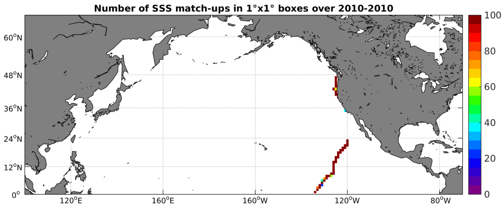
Figure 4: Number of SSS match-ups between TSG-GOSUD-Sailing-ship SSS and the SMOS-L3-CATDS-CPDC-V3-10DAYS-25KM SSS product for the North Pacific Ocean Pi-MEP region over 1^\circ \times 1^\circ boxes and for the full satellite product period.
