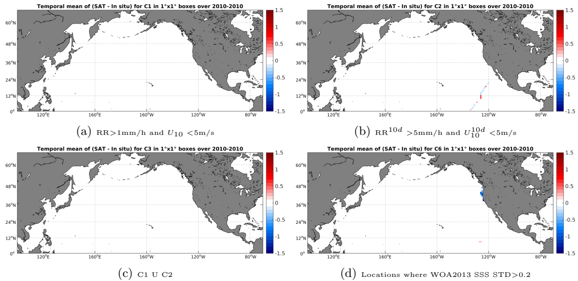
Figure 12: Temporal mean gridded over spatial boxes of size 1^\circ \times 1^\circ of \Delta SSS (SMOS-L3-CATDS-CPDC-V3-10DAYS-25KM - TSG-GOSUD-Sailing-ship) for 4 different subdatasets corresponding to: RR > 1\text{mm/h} and U_{10} < 5\text{m/s} (a), RR^{10d} > 5\text{mm/h} and U_{10}^{10d} < 5\text{m/s} (b), C1 U C2 (c), Locations where WOA2013 SSS STD > 0.2 (d).
