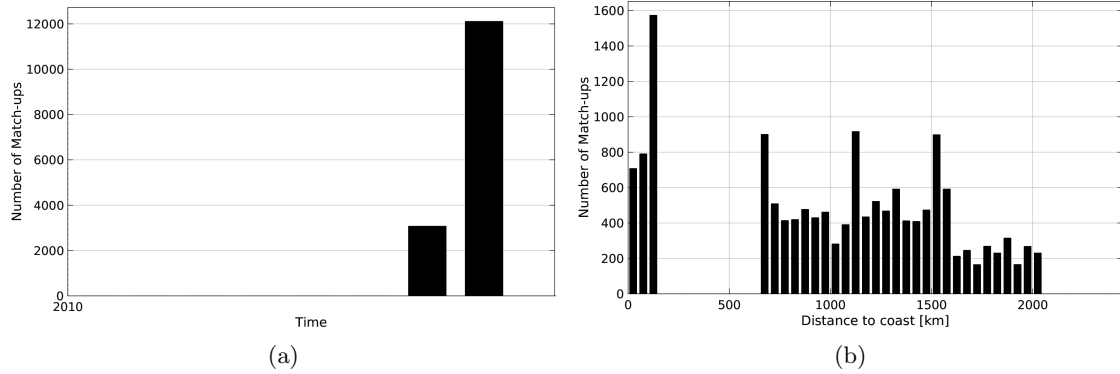
Figure 1: Number of match-ups between TSG-GOSUD-Sailing-ship and SMOS-L3-CATDS-CPDC-V3-10DAYS-25KM SSS as a function of time (a) and as function of the distance to coast (b) over the North Pacific Ocean Pi-MEP region and for the full satellite product period.
