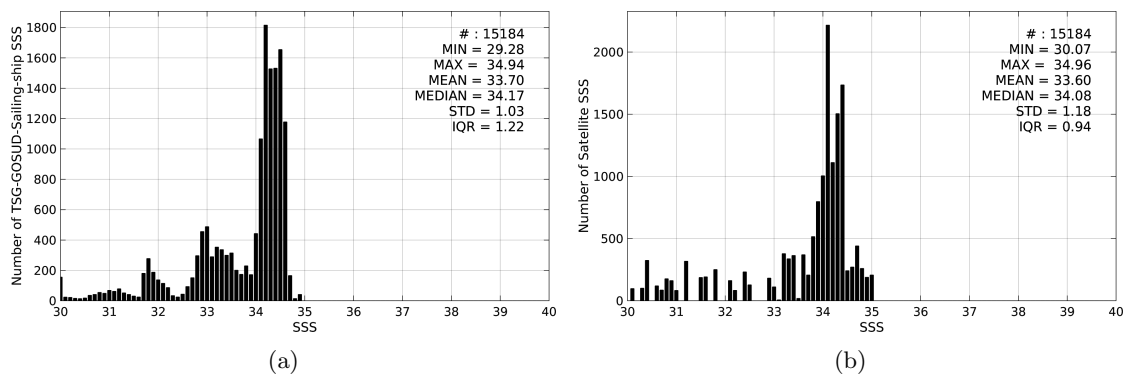
Figure 2: Histograms of SSS from TSG-GOSUD-Sailing-ship (a) and SMOS-L3-CATDS-CPDC-V3-10DAYS-25KM (b) considering all match-up pairs per bins of 0.1 over the North Pacific Ocean Pi-MEP region and for the full satellite product period.
