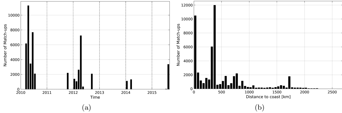
Figure 1: Number of match-ups between TSG-GOSUD-Research-vessel and SMOS-L3-CATDS-CPDC-V3-10DAYS-25KM SSS as a function of time (a) and as function of the distance to coast (b) over the North Pacific Ocean Pi-MEP region and for the full satellite product period.
