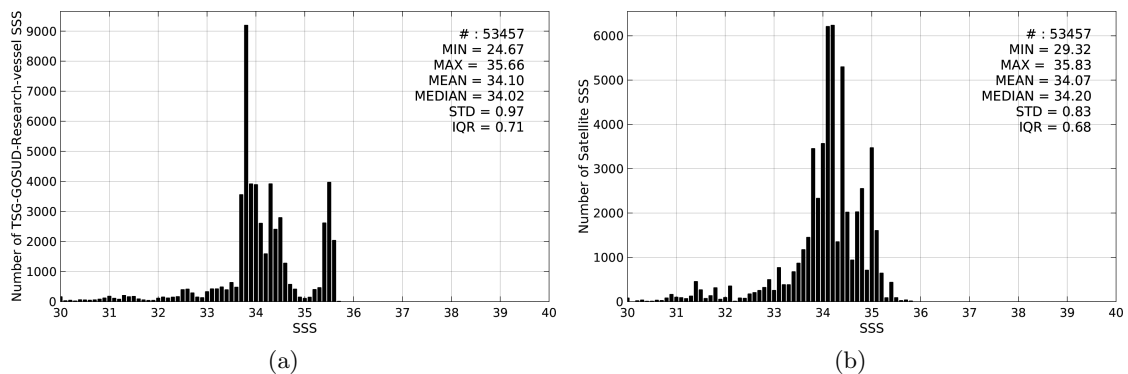
Figure 2: Histograms of SSS from TSG-GOSUD-Research-vessel (a) and SMOS-L3-CATDS-CPDC-V3-10DAYS-25KM (b) considering all match-up pairs per bins of 0.1 over the North Pacific Ocean Pi-MEP region and for the full satellite product period.
