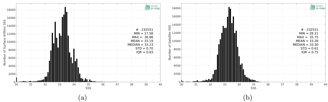
Figure 2: Histograms of SSS from Surface drifters (a) and SMOS-L3-CATDS-CPDC-V3-10DAYS-25KM (b) considering all match-up pairs per bins of 0.1 over the North Pacific Ocean Pi-MEP region and for the full satellite product period.
