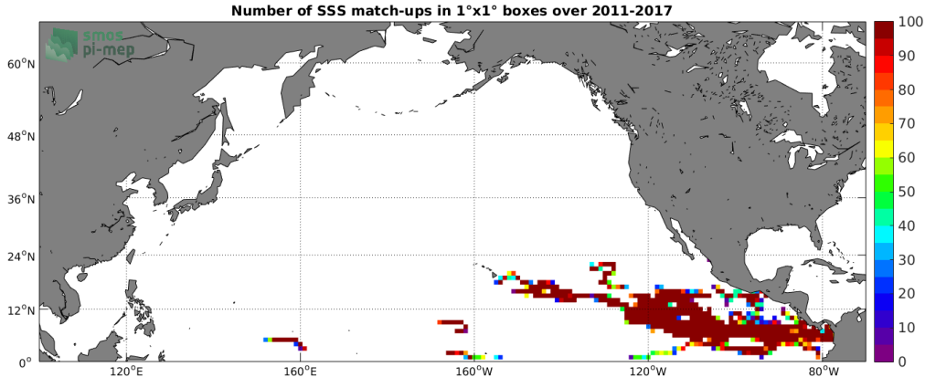
Figure 3: Number of SSS match-ups between Surface drifters SSS and the SMOS-L3-CATDS-CPDC-V3-10DAYS-25KM SSS product for the North Pacific Ocean Pi-MEP region over 1°x1° boxes and for the full satellite product period.
