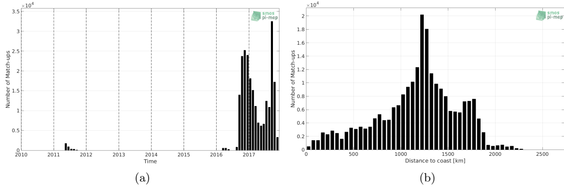
Figure 1: Number of match-ups between Surface drifters and SMOS-L3-CATDS-CPDC-V3-10DAYS-25KM SSS as a function of time (a) and as function of the distance to coast (b) over the North Pacific Ocean Pi-MEP region and for the full satellite product period.
