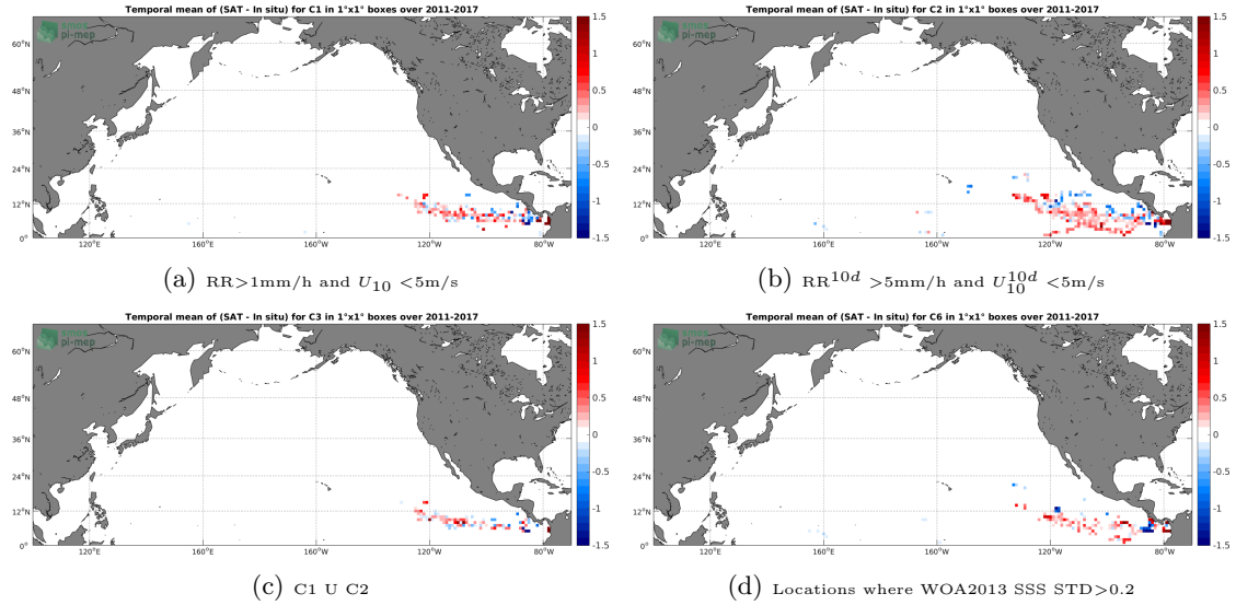
Figure 11: Temporal mean gridded over spatial boxes of size 1^\circ \times 1^\circ of \Delta SSS (SMOS-L3-CATDS-CPDC-V3-10DAYS-25KM - Surface drifters) for 4 different subdatasets corresponding to: RR > 1\text{mm/h} and U_{10} < 5\text{m/s} (a), RR^{10d} > 5\text{mm/h} and U_{10}^{10d} < 5\text{m/s} (b), C1 U C2 (c), Locations where WOA2013 SSS STD > 0.2 (d).
