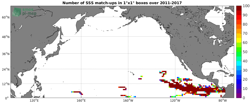
Figure 3: Number of SSS match-ups between Surface drifters SSS and the SMOS-L3-CATDS-CPDC-V3-10DAYS-25KM SSS product for the North Pacific Ocean Pi-MEP region over 1^\circ \times 1^\circ boxes and for the full satellite product period.
