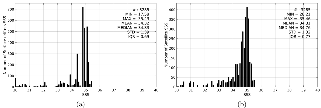
Figure 2: Histograms of SSS from Surface drifters (a) and SMOS-L3-CATDS-CPDC-V3-10DAYS-25KM (b) considering all match-up pairs per bins of 0.1 over the North Pacific Ocean Pi-MEP region and for the full satellite product period.
