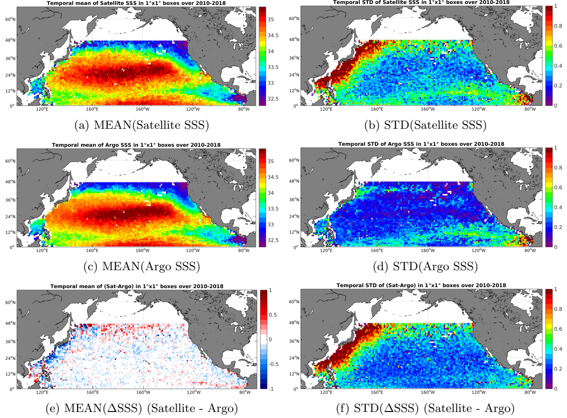
Figure 6: Temporal mean (left) and STD (right) of SSS from SMOS-L3-CATDS-CPDC-V3-10DAYS-25KM (top), Argo (middle), and of \Delta\text{SSS} (Satellite - Argo). Only match-up pairs are used to generate these maps.
