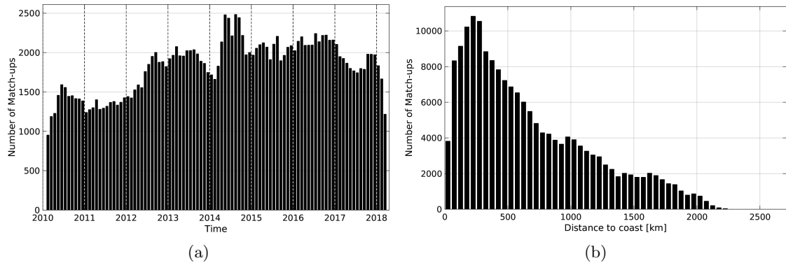
Figure 1: Number of match-ups between Argo and SMOS-L3-CATDS-CPDC-V3-10DAYS-25KM SSS as a function of time (a) and as function of the distance to coast (b) over the North Pacific Ocean Pi-MEP region and for the full satellite product period.
