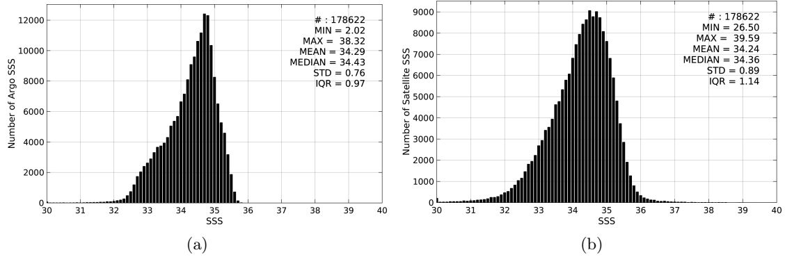
Figure 2: Histograms of SSS from Argo (a) and SMOS-L3-CATDS-CPDC-V3-10DAYS-25KM (b) considering all match-up pairs per bins of 0.1 over the North Pacific Ocean Pi-MEP region and for the full satellite product period.
