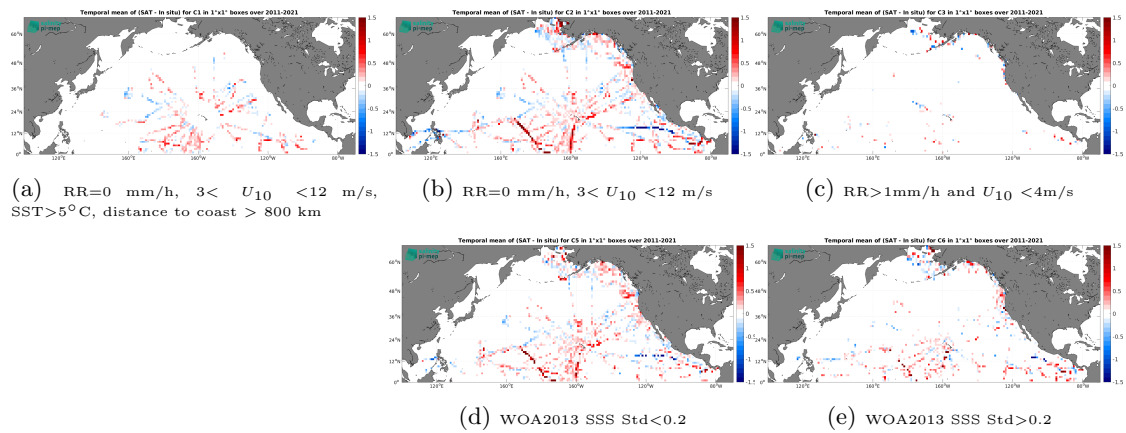
Figure 14: Temporal mean gridded over spatial boxes of size 1^\circ \times 1^\circ of \Delta SSS (SMOS SSS L3 v2 - 9-Days (BEC) - TSG (SAMOS)) for 5 different subdatasets corresponding to:RR=0 mm/h, 3 < U_{10} < 12 m/s, SST >5^\circ\text{C} , distance to coast > 800 km (a), RR=0 mm/h, 3 < U_{10} < 12 m/s (b), RR >1 mm/h and U_{10} < 4 m/s (c), WOA2013 SSS Std <0.2 (d), WOA2013 SSS Std >0.2 (e).
