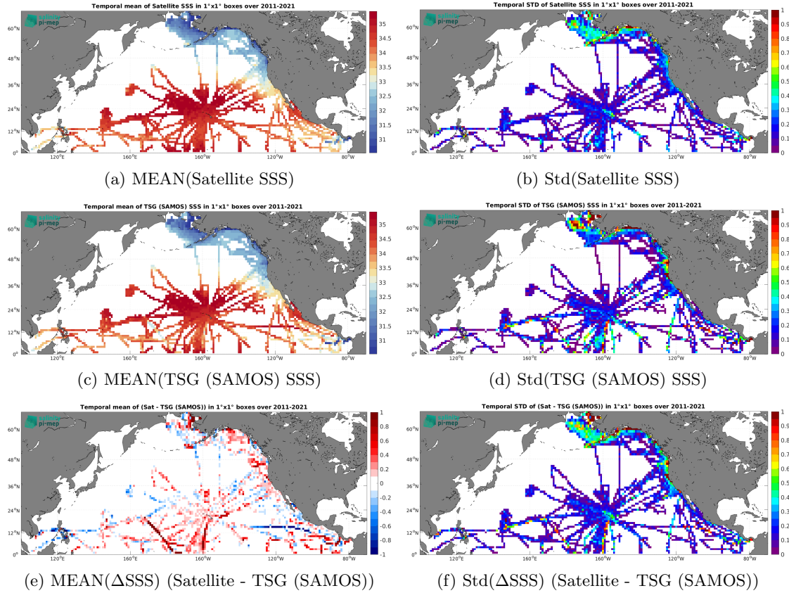
Figure 7: Temporal mean (left) and Std (right) of SSS from SMOS SSS L3 v2 - 9-Days (BEC) (top), TSG (SAMOS) (middle), and of \Delta\text{SSS} (Satellite - TSG (SAMOS)). Only match-up pairs are used to generate these maps.
