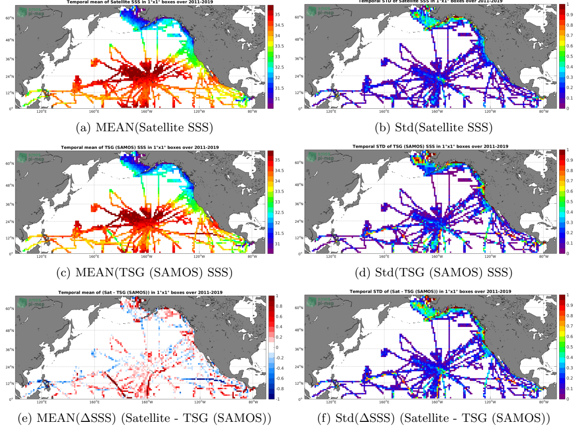
Figure 6: Temporal mean (left) and Std (right) of SSS from SMOS SSS L3 v2 - 9-Days (BEC) (top), TSG (SAMOS) (middle), and of \Delta\text{SSS} (Satellite - TSG (SAMOS)). Only match-up pairs are used to generate these maps.
