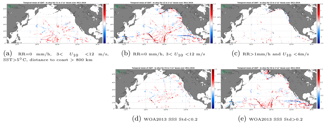
Figure 12: Temporal mean gridded over spatial boxes of size 1^\circ \times 1^\circ of \Delta SSS (SMOS SSS L3 v2 - 9-Days (BEC) - TSG (SAMOS)) for 5 different subdatasets corresponding to: RR=0 mm/h, 3 < U_{10} < 12 m/s, SST > 5^\circ C , distance to coast > 800 km (a), RR=0 mm/h, 3 < U_{10} < 12 m/s (b), RR > 1 mm/h and U_{10} < 4 m/s (c), WOA2013 SSS Std < 0.2 (d), WOA2013 SSS Std > 0.2 (e).
