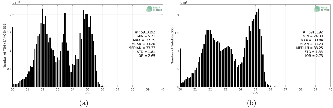
Figure 2: Histograms of SSS from TSG (SAMOS) (a) and SMOS SSS L3 v2 - 9-Days (BEC) (b) considering all match-up pairs per bins of 0.1 over the North Pacific Ocean Pi-MEP region and for the full satellite product period.
