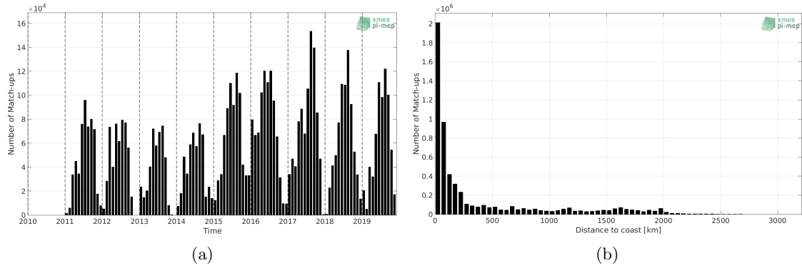
Figure 1: Number of match-ups between TSG (SAMOS) and SMOS SSS L3 v2 - 9-Days (BEC) SSS as a function of time (a) and as function of the distance to coast (b) over the North Pacific Ocean Pi-MEP region and for the full satellite product period.
