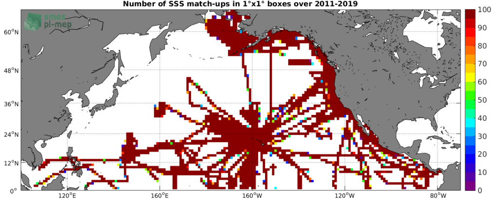
Figure 4: Number of SSS match-ups between TSG (SAMOS) SSS and the SMOS SSS L3 v2 - 9-Days (BEC) SSS product for the North Pacific Ocean Pi-MEP region over 1^\circ \times 1^\circ boxes and for the full satellite product period.
