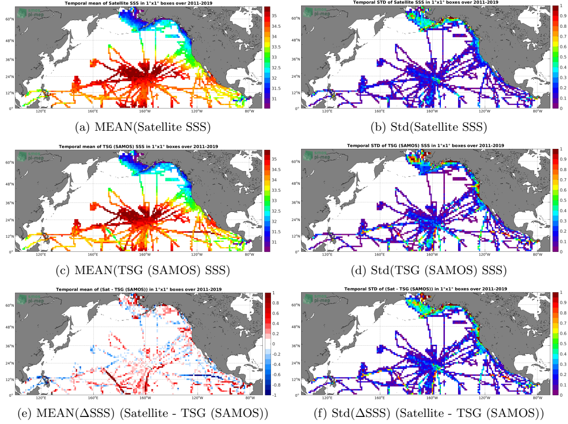
Figure 6: Temporal mean (left) and Std (right) of SSS from SMOS SSS L3 v2 - 9-Days (BEC) (top), TSG (SAMOS) (middle), and of \Delta SSS (Satellite - TSG (SAMOS)). Only match-up pairs are used to generate these maps.
