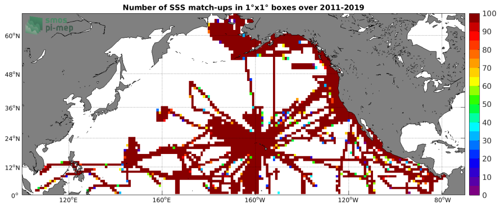
Figure 4: Number of SSS match-ups between TSG (SAMOS) SSS and the SMOS SSS L3 v2 - 9-Days (BEC) SSS product for the North Pacific Ocean Pi-MEP region over 1°x1° boxes and for the full satellite product period.
