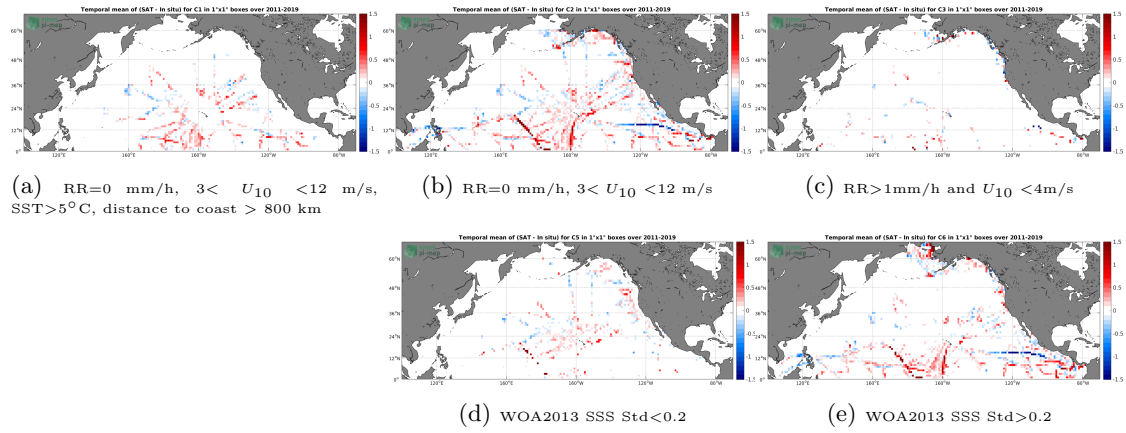
Figure 12: Temporal mean gridded over spatial boxes of size 1^\circ \times 1^\circ of \Delta SSS (SMOS L3 v2 - 9-Days (BEC) - TSG (SAMOS)) for 5 different subdatasets corresponding to:RR=0 mm/h, 3 < U_{10} < 12 m/s, SST >5^\circ\text{C} , distance to coast > 800 km (a), RR=0 mm/h, 3 < U_{10} < 12 m/s (b), RR >1 mm/h and U_{10} < 4 m/s (c), WOA2013 SSS Std <0.2 (d), WOA2013 SSS Std >0.2 (e).
