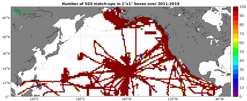
Figure 4: Number of SSS match-ups between TSG (SAMOS) SSS and the SMOS L3 v2 - 9-Days (BEC) SSS product for the North Pacific Ocean Pi-MEP region over 1^\circ \times 1^\circ boxes and for the full satellite product period.
