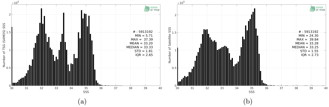
Figure 2: Histograms of SSS from TSG (SAMOS) (a) and SMOS L3 v2 - 9-Days (BEC) (b) considering all match-up pairs per bins of 0.1 over the North Pacific Ocean Pi-MEP region and for the full satellite product period.
