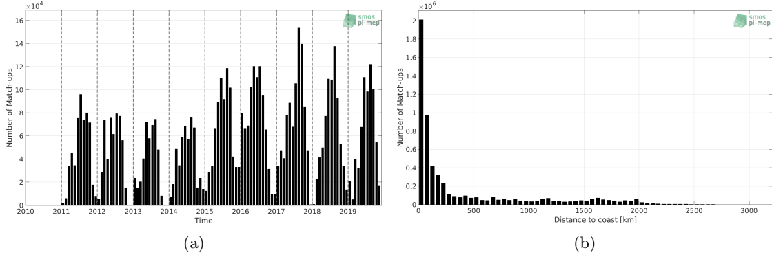
Figure 1: Number of match-ups between TSG (SAMOS) and SMOS L3 v2 - 9-Days (BEC) SSS as a function of time (a) and as function of the distance to coast (b) over the North Pacific Ocean Pi-MEP region and for the full satellite product period.
