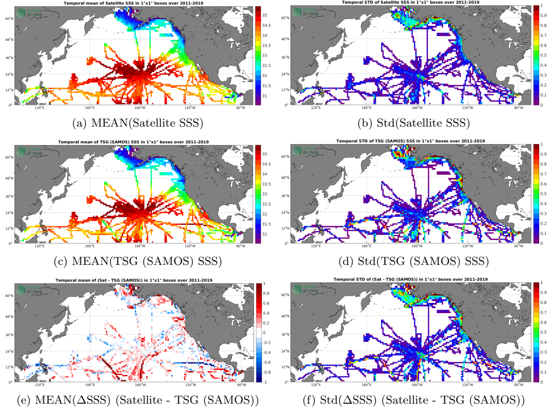
Figure 6: Temporal mean (left) and Std (right) of SSS from SMOS L3 v2 - 9-Days (BEC) (top), TSG (SAMOS) (middle), and of \Delta SSS (Satellite - TSG (SAMOS)). Only match-up pairs are used to generate these maps.
