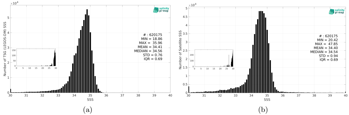
Figure 3: Histograms of SSS from TSG (LEGOS-DM) (a) and SMOS SSS L3 v2 - 9-Days (BEC) (b) considering all match-up pairs per bins of 0.1 over the North Pacific Ocean Pi-MEP region and for the full satellite product period.
