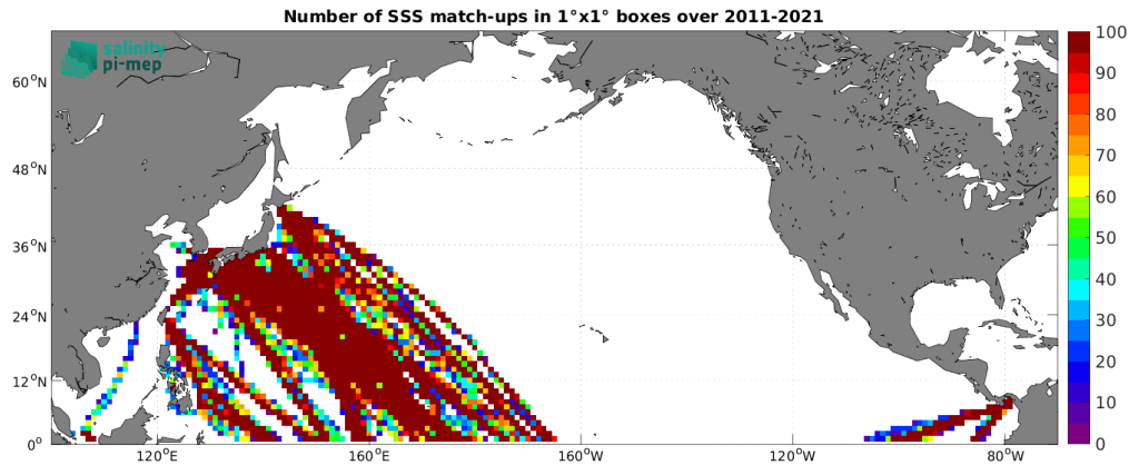
Figure 5: Number of SSS match-ups between TSG (LEGOS-DM) SSS and the SMOS SSS L3 v2 - 9-Days (BEC) SSS product for the North Pacific Ocean Pi-MEP region over 1^\circ \times 1^\circ boxes and for the full satellite product period.
