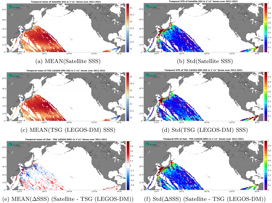
Figure 7: Temporal mean (left) and Std (right) of SSS from SMOS SSS L3 v2 - 9-Days (BEC) (top), TSG (LEGOS-DM) ( in situ ) dataset (middle), and of \Delta\text{SSS} (Satellite - TSG (LEGOS-DM)). Only match-up pairs are used to generate these maps.
