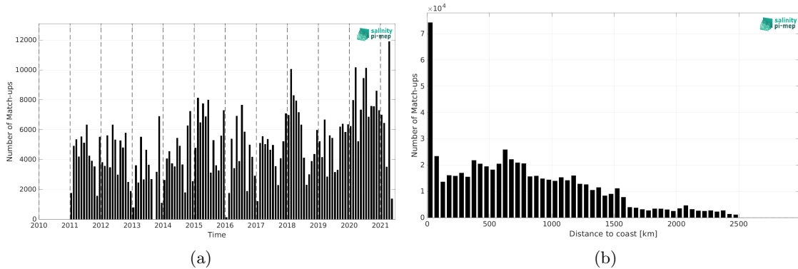
Figure 2: Number of match-ups between TSG (LEGOS-DM) and SMOS SSS L3 v2 - 9-Days (BEC) SSS as a function of time (a) and as function of the distance to coast (b) over the North Pacific Ocean Pi-MEP region and for the full satellite product period.
