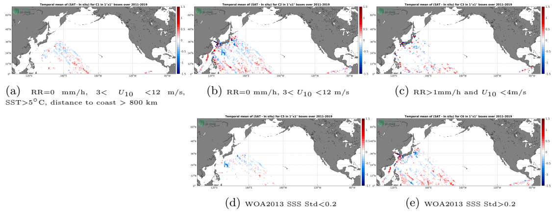
Figure 12: Temporal mean gridded over spatial boxes of size 1^\circ \times 1^\circ of \Delta SSS (SMOS SSS L3 v2 - 9-Days (BEC) - TSG (LEGOS-DM)) for 5 different subdatasets corresponding to: RR=0 mm/h, 3 < U_{10} < 12 m/s, SST > 5^\circ C , distance to coast > 800 km (a), RR=0 mm/h, 3 < U_{10} < 12 m/s (b), RR > 1 mm/h and U_{10} < 4 m/s (c), WOA2013 SSS Std < 0.2 (d), WOA2013 SSS Std > 0.2 (e).
