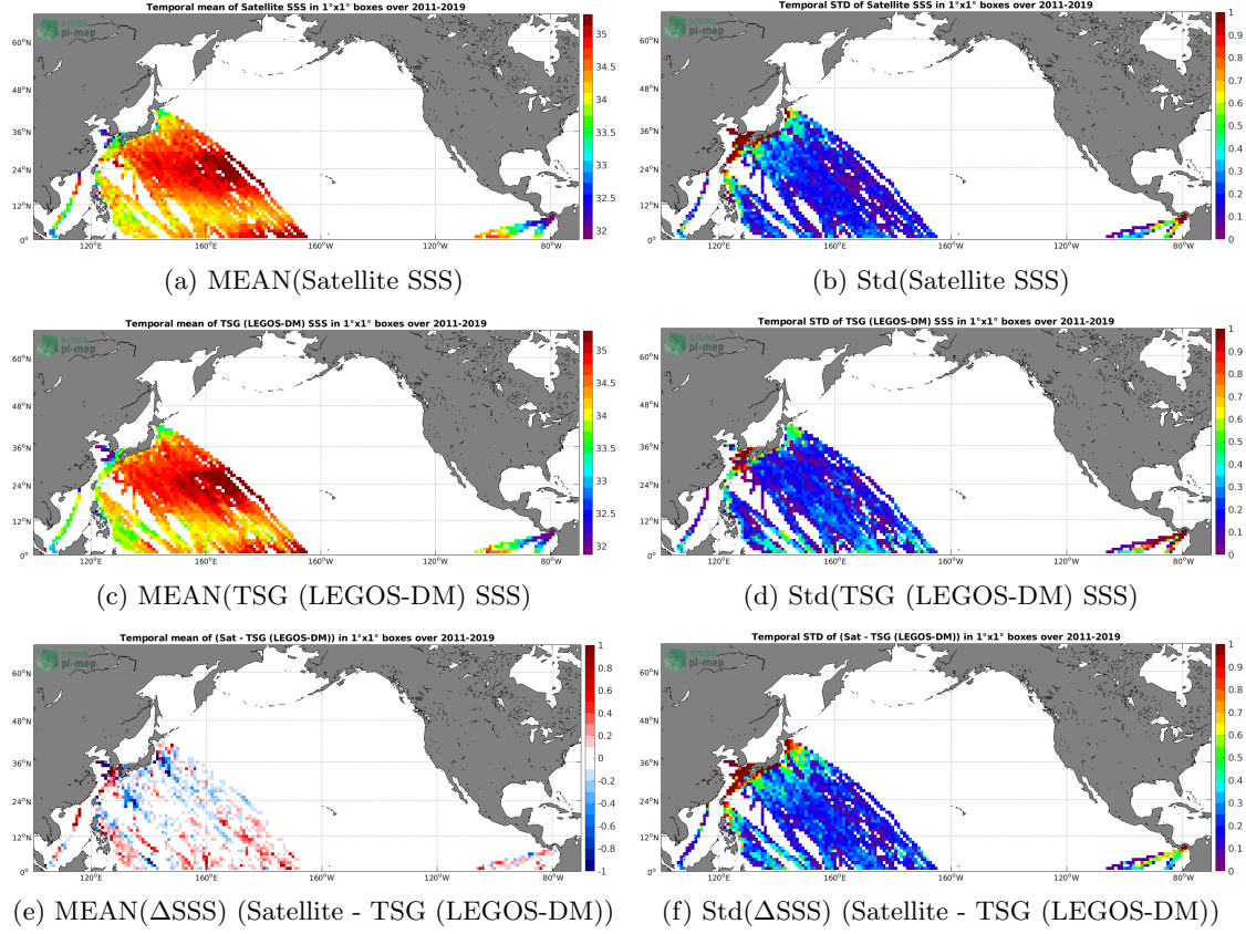
Figure 6: Temporal mean (left) and Std (right) of SSS from SMOS SSS L3 v2 - 9-Days (BEC) (top), TSG (LEGOS-DM) (middle), and of \Delta SSS (Satellite - TSG (LEGOS-DM)). Only match-up pairs are used to generate these maps.
