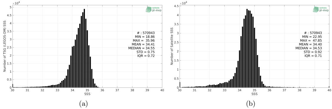
Figure 2: Histograms of SSS from TSG (LEGOS-DM) (a) and SMOS SSS L3 v2 - 9-Days (BEC) (b) considering all match-up pairs per bins of 0.1 over the North Pacific Ocean Pi-MEP region and for the full satellite product period.
