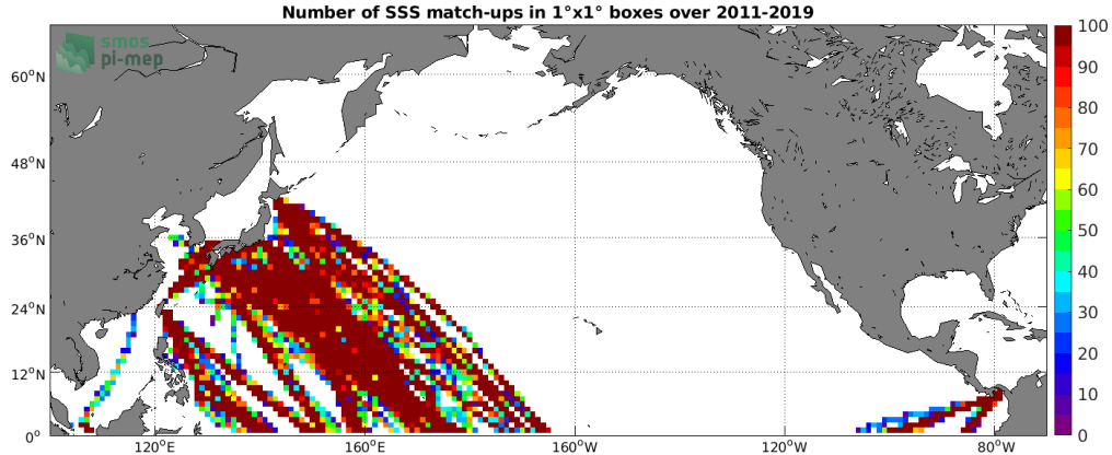
Figure 4: Number of SSS match-ups between TSG (LEGOS-DM) SSS and the SMOS SSS L3 v2 - 9-Days (BEC) SSS product for the North Pacific Ocean Pi-MEP region over 1^\circ \times 1^\circ boxes and for the full satellite product period.
