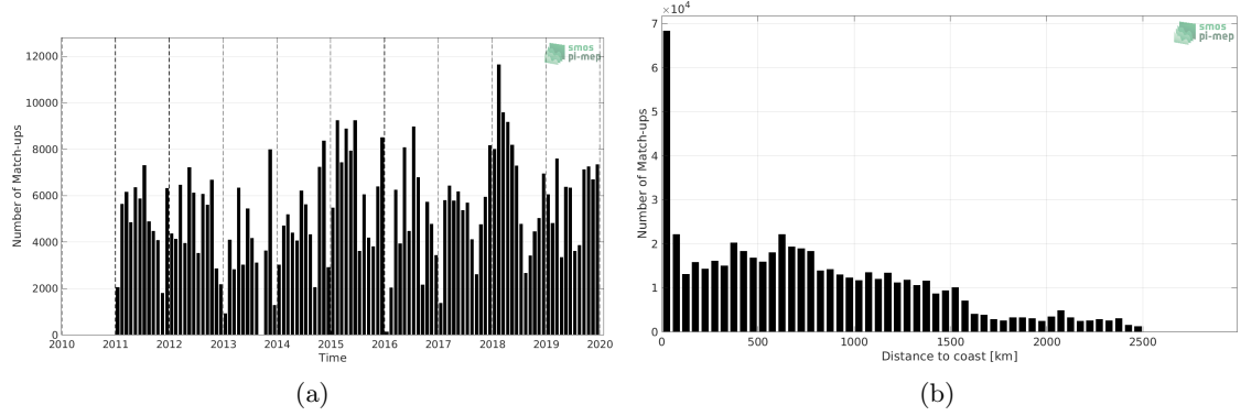
Figure 1: Number of match-ups between TSG (LEGOS-DM) and SMOS SSS L3 v2 - 9-Days (BEC) SSS as a function of time (a) and as function of the distance to coast (b) over the North Pacific Ocean Pi-MEP region and for the full satellite product period.
