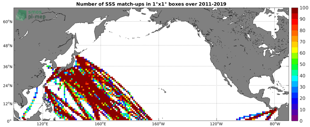
Figure 4: Number of SSS match-ups between TSG (LEGOS-DM) SSS and the SMOS SSS L3 v2 - 9-Days (BEC) SSS product for the North Pacific Ocean Pi-MEP region over 1°x1° boxes and for the full satellite product period.
