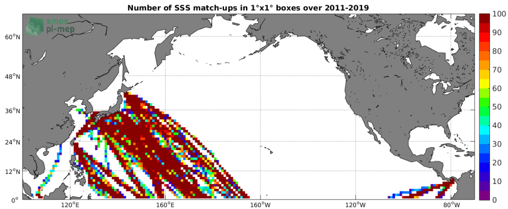
Figure 4: Number of SSS match-ups between TSG (LEGOS-DM) SSS and the SMOS L3 v2 - 9-Days (BEC) SSS product for the North Pacific Ocean Pi-MEP region over 1^\circ \times 1^\circ boxes and for the full satellite product period.
