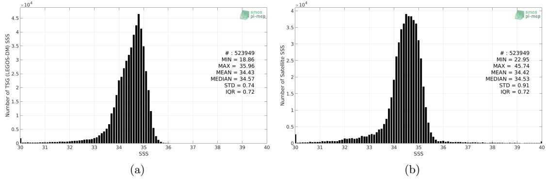
Figure 2: Histograms of SSS from TSG (LEGOS-DM) (a) and SMOS L3 v2 - 9-Days (BEC) (b) considering all match-up pairs per bins of 0.1 over the North Pacific Ocean Pi-MEP region and for the full satellite product period.
