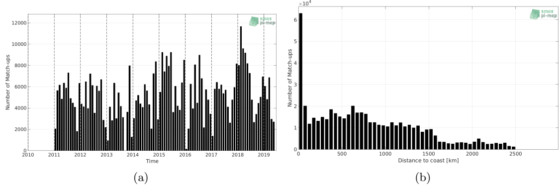
Figure 1: Number of match-ups between TSG (LEGOS-DM) and SMOS L3 v2 - 9-Days (BEC) SSS as a function of time (a) and as function of the distance to coast (b) over the North Pacific Ocean Pi-MEP region and for the full satellite product period.
