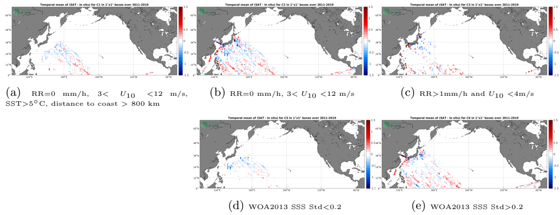
Figure 12: Temporal mean gridded over spatial boxes of size 1^\circ \times 1^\circ of \Delta SSS (SMOS L3 v2 - 9-Days (BEC) - TSG (LEGOS-DM)) for 5 different subdatasets corresponding to: RR=0 mm/h, 3 < U_{10} < 12 m/s, SST > 5^\circ C , distance to coast > 800 km (a), RR=0 mm/h, 3 < U_{10} < 12 m/s (b), RR > 1 mm/h and U_{10} < 4 m/s (c), WOA2013 SSS Std < 0.2 (d), WOA2013 SSS Std > 0.2 (e).
