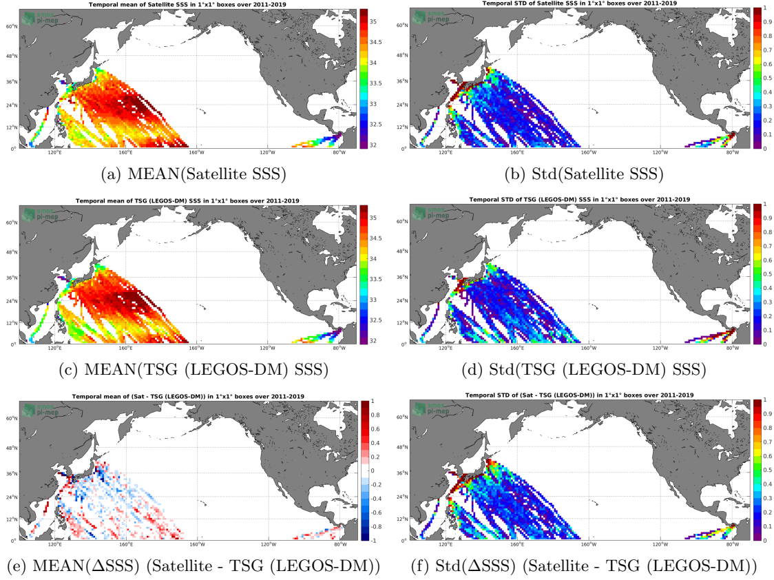
Figure 6: Temporal mean (left) and Std (right) of SSS from SMOS L3 v2 - 9-Days (BEC) (top), TSG (LEGOS-DM) (middle), and of \Delta SSS (Satellite - TSG (LEGOS-DM)). Only match-up pairs are used to generate these maps.
