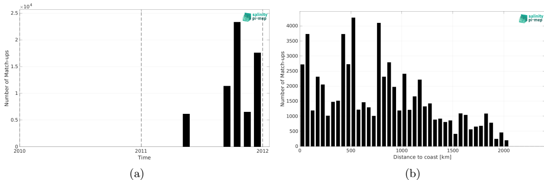
Figure 2: Number of match-ups between TSG (GOSUD-Sailing-ship) and SMOS SSS L3 v2 - 9-Days (BEC) SSS as a function of time (a) and as function of the distance to coast (b) over the North Pacific Ocean Pi-MEP region and for the full satellite product period.
