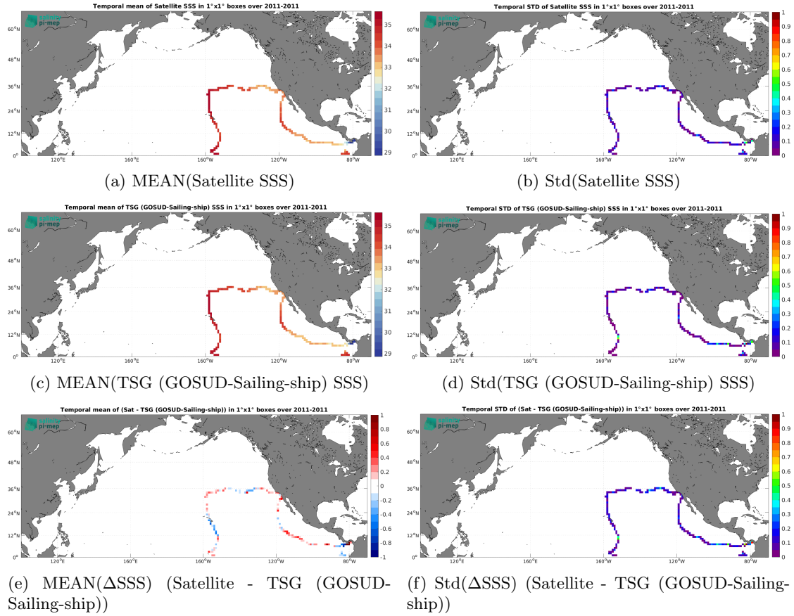
Figure 7: Temporal mean (left) and Std (right) of SSS from SMOS SSS L3 v2 - 9-Days (BEC) (top), TSG (GOSUD-Sailing-ship) (middle), and of \Delta SSS (Satellite - TSG (GOSUD-Sailing-ship)). Only match-up pairs are used to generate these maps.
