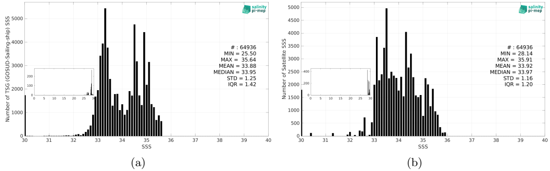
Figure 3: Histograms of SSS from TSG (GOSUD-Sailing-ship) (a) and SMOS SSS L3 v2 - 9-Days (BEC) (b) considering all match-up pairs per bins of 0.1 over the North Pacific Ocean Pi-MEP region and for the full satellite product period.
