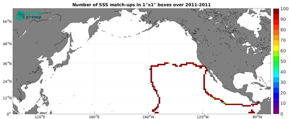
Figure 5: Number of SSS match-ups between TSG (GOSUD-Sailing-ship) SSS and the SMOS SSS L3 v2 - 9-Days (BEC) SSS product for the North Pacific Ocean Pi-MEP region over 1^\circ \times 1^\circ boxes and for the full satellite product period.
