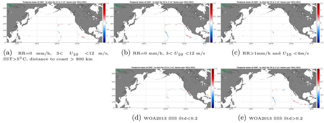
Figure 12: Temporal mean gridded over spatial boxes of size 1^\circ \times 1^\circ of \Delta SSS (SMOS SSS L3 v2 - 9-Days (BEC) - TSG (GOSUD-Sailing-ship)) for 5 different subdatasets corresponding to: RR=0 mm/h, 3 < U_{10} < 12 m/s, SST>5°C, distance to coast > 800 km (a), RR=0 mm/h, 3 < U_{10} < 12 m/s (b), RR>1mm/h and U_{10} < 4 m/s (c), WOA2013 SSS Std<0.2 (d), WOA2013 SSS Std>0.2 (e).
