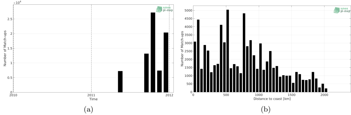
Figure 1: Number of match-ups between TSG (GOSUD-Sailing-ship) and SMOS SSS L3 v2 - 9-Days (BEC) SSS as a function of time (a) and as function of the distance to coast (b) over the North Pacific Ocean Pi-MEP region and for the full satellite product period.
