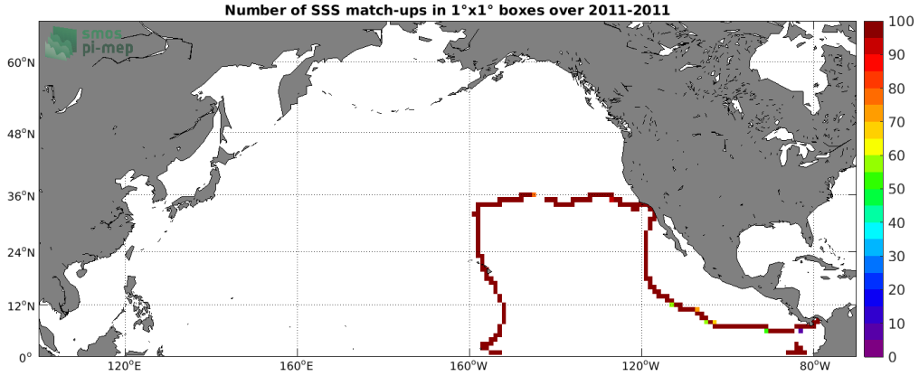
Figure 4: Number of SSS match-ups between TSG (GOSUD-Sailing-ship) SSS and the SMOS SSS L3 v2 - 9-Days (BEC) SSS product for the North Pacific Ocean Pi-MEP region over 1^\circ \times 1^\circ boxes and for the full satellite product period.
