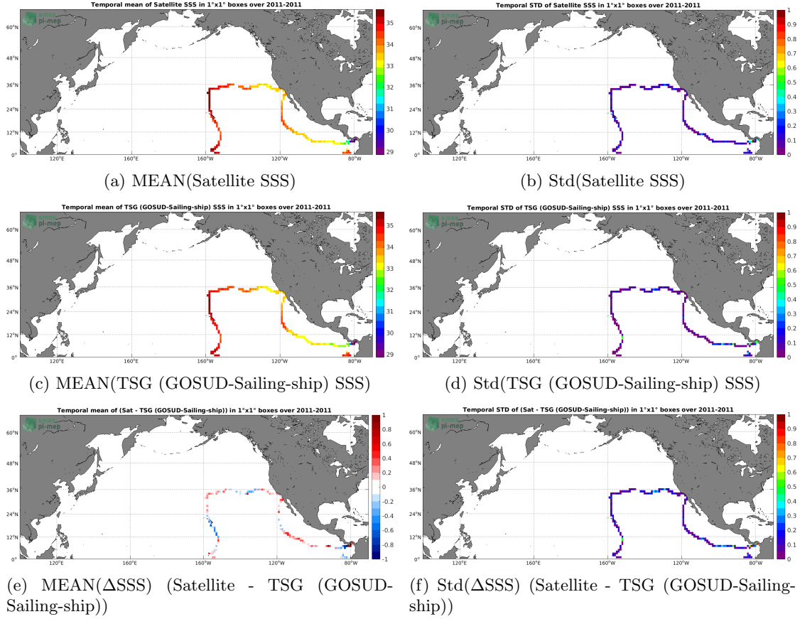
Figure 6: Temporal mean (left) and Std (right) of SSS from SMOS SSS L3 v2 - 9-Days (BEC) (top), TSG (GOSUD-Sailing-ship) (middle), and of \Delta SSS (Satellite - TSG (GOSUD-Sailing-ship)). Only match-up pairs are used to generate these maps.
