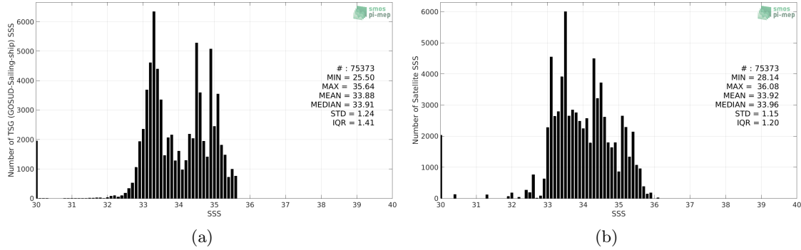
Figure 2: Histograms of SSS from TSG (GOSUD-Sailing-ship) (a) and SMOS SSS L3 v2 - 9-Days (BEC) (b) considering all match-up pairs per bins of 0.1 over the North Pacific Ocean Pi-MEP region and for the full satellite product period.
