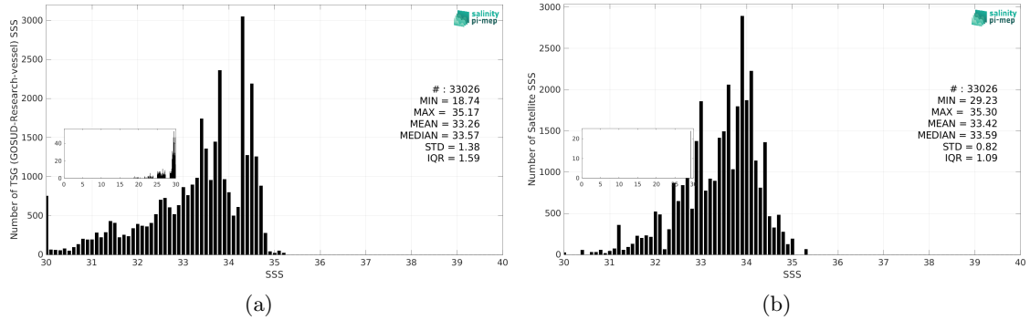
Figure 3: Histograms of SSS from TSG (GOSUD-Research-vessel) (a) and SMOS SSS L3 v2 - 9-Days (BEC) (b) considering all match-up pairs per bins of 0.1 over the North Pacific Ocean Pi-MEP region and for the full satellite product period.
