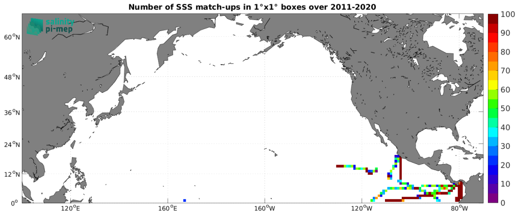
Figure 5: Number of SSS match-ups between TSG (GOSUD-Research-vessel) SSS and the SMOS SSS L3 v2 - 9-Days (BEC) SSS product for the North Pacific Ocean Pi-MEP region over 1^\circ \times 1^\circ boxes and for the full satellite product period.
