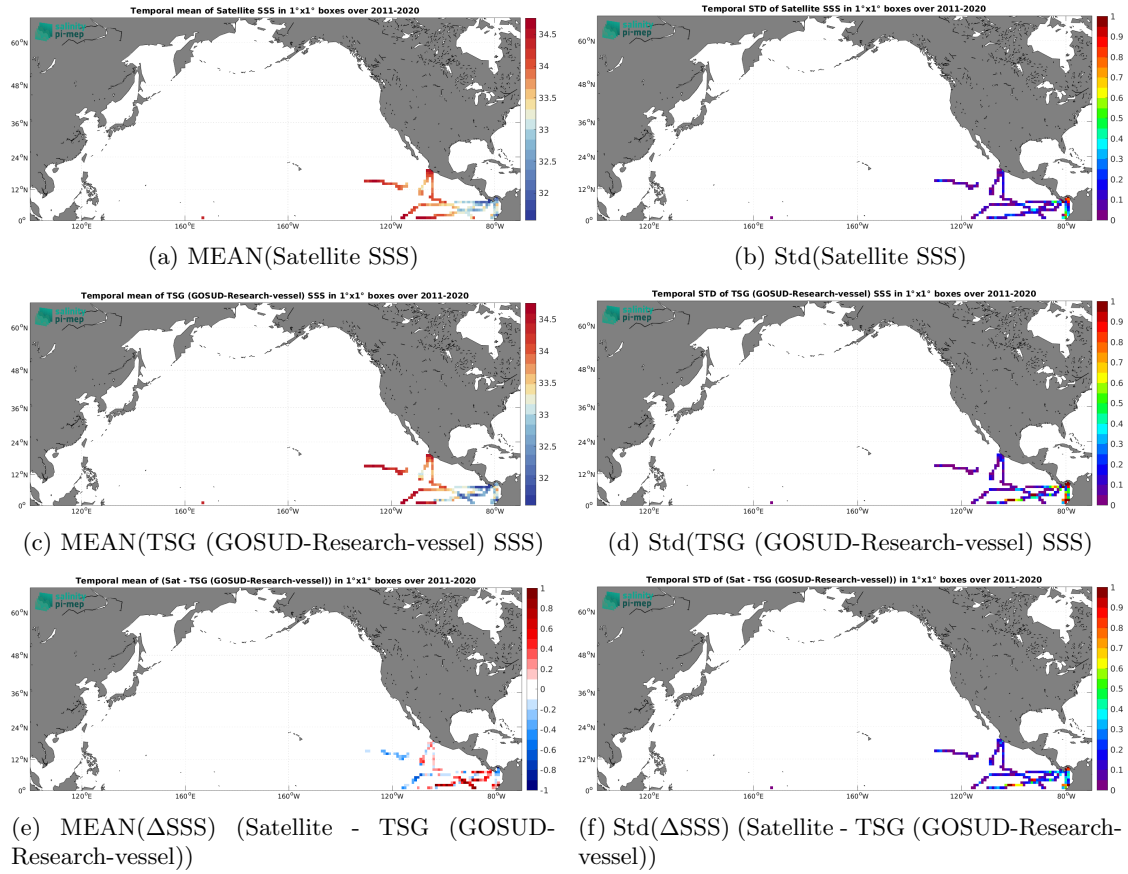
Figure 7: Temporal mean (left) and Std (right) of SSS from SMOS SSS L3 v2 - 9-Days (BEC) (top), TSG (GOSUD-Research-vessel) (middle), and of \Delta SSS (Satellite - TSG (GOSUD-Research-vessel)). Only match-up pairs are used to generate these maps.
