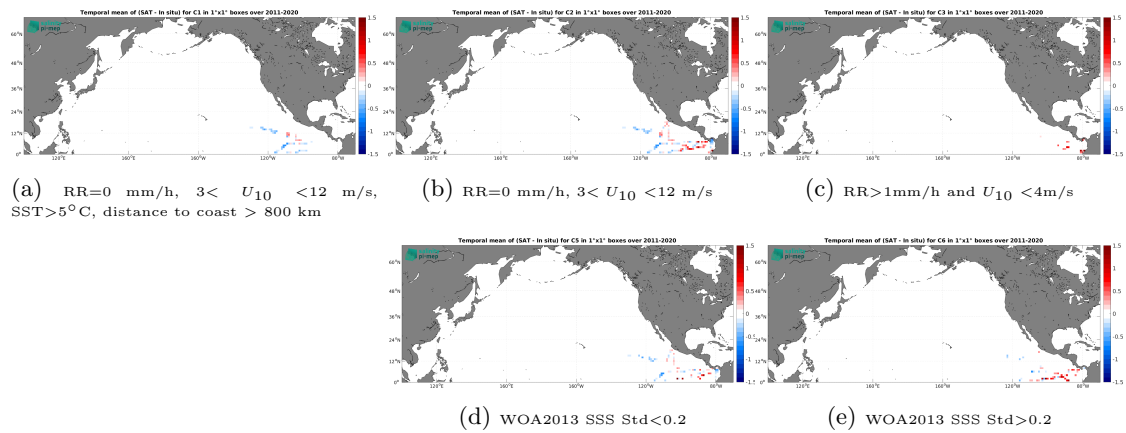
Figure 14: Temporal mean gridded over spatial boxes of size 1^\circ \times 1^\circ of \Delta SSS (SMOS SSS L3 v2 - 9-Days (BEC) - TSG (GOSUD-Research-vessel)) for 5 different subdatasets corresponding to:RR=0 mm/h, 3 < U_{10} < 12 m/s, SST >5^\circ\text{C} , distance to coast > 800 km (a), RR=0 mm/h, 3 < U_{10} < 12 m/s (b), RR >1 mm/h and U_{10} < 4 m/s (c), WOA2013 SSS Std <0.2 (d), WOA2013 SSS Std >0.2 (e).
