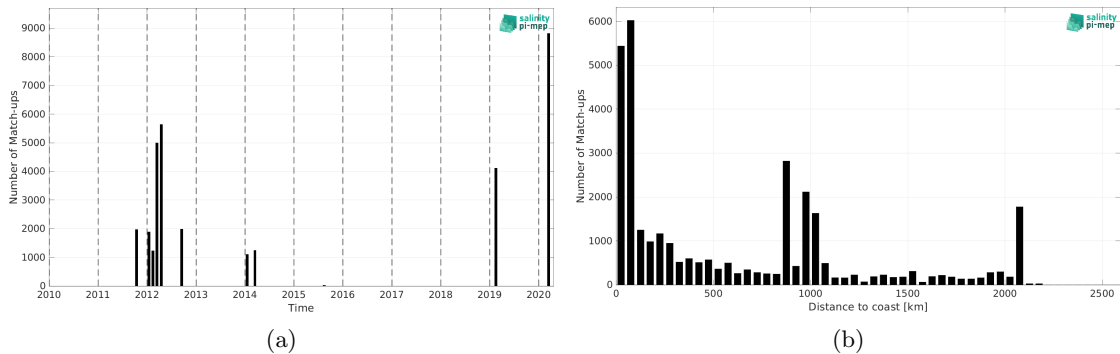
Figure 2: Number of match-ups between TSG (GOSUD-Research-vessel) and SMOS SSS L3 v2 - 9-Days (BEC) SSS as a function of time (a) and as function of the distance to coast (b) over the North Pacific Ocean Pi-MEP region and for the full satellite product period.
