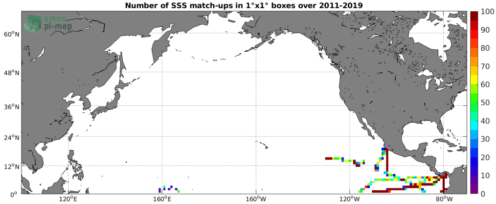
Figure 4: Number of SSS match-ups between TSG (GOSUD-Research-vessel) SSS and the SMOS SSS L3 v2 - 9-Days (BEC) SSS product for the North Pacific Ocean Pi-MEP region over 1^\circ \times 1^\circ boxes and for the full satellite product period.
