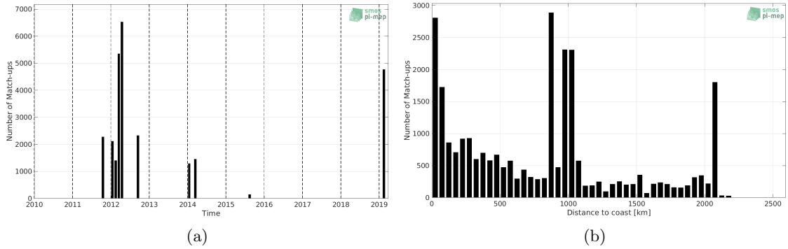
Figure 1: Number of match-ups between TSG (GOSUD-Research-vessel) and SMOS SSS L3 v2 - 9-Days (BEC) SSS as a function of time (a) and as function of the distance to coast (b) over the North Pacific Ocean Pi-MEP region and for the full satellite product period.
