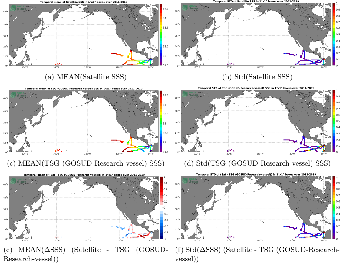
Figure 6: Temporal mean (left) and Std (right) of SSS from SMOS SSS L3 v2 - 9-Days (BEC) (top), TSG (GOSUD-Research-vessel) (middle), and of \Delta SSS (Satellite - TSG (GOSUD-Research-vessel)). Only match-up pairs are used to generate these maps.
