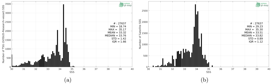
Figure 2: Histograms of SSS from TSG (GOSUD-Research-vessel) (a) and SMOS SSS L3 v2 - 9-Days (BEC) (b) considering all match-up pairs per bins of 0.1 over the North Pacific Ocean Pi-MEP region and for the full satellite product period.
