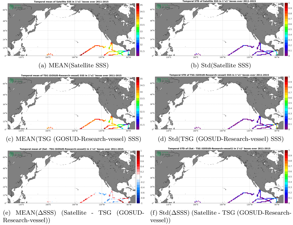
Figure 6: Temporal mean (left) and Std (right) of SSS from SMOS L3 v2 - 9-Days (BEC) (top), TSG (GOSUD-Research-vessel) (middle), and of \Delta SSS (Satellite - TSG (GOSUD-Research-vessel)). Only match-up pairs are used to generate these maps.
