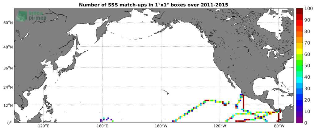
Figure 4: Number of SSS match-ups between TSG (GOSUD-Research-vessel) SSS and the SMOS L3 v2 - 9-Days (BEC) SSS product for the North Pacific Ocean Pi-MEP region over 1^\circ \times 1^\circ boxes and for the full satellite product period.
