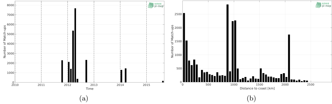
Figure 1: Number of match-ups between TSG (GOSUD-Research-vessel) and SMOS L3 v2 - 9-Days (BEC) SSS as a function of time (a) and as function of the distance to coast (b) over the North Pacific Ocean Pi-MEP region and for the full satellite product period.
