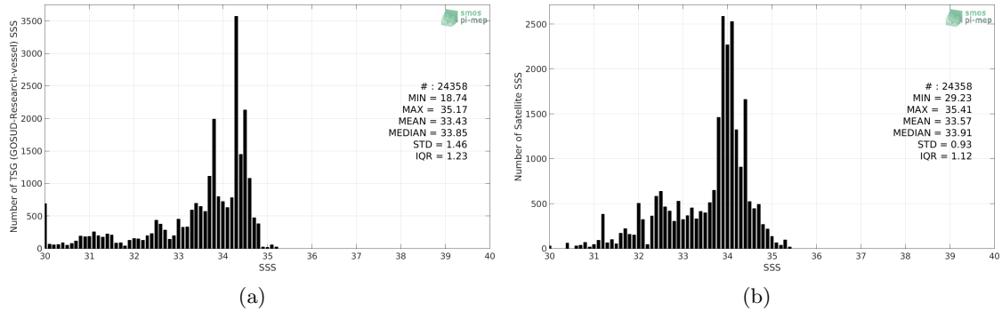
Figure 2: Histograms of SSS from TSG (GOSUD-Research-vessel) (a) and SMOS L3 v2 - 9-Days (BEC) (b) considering all match-up pairs per bins of 0.1 over the North Pacific Ocean Pi-MEP region and for the full satellite product period.
