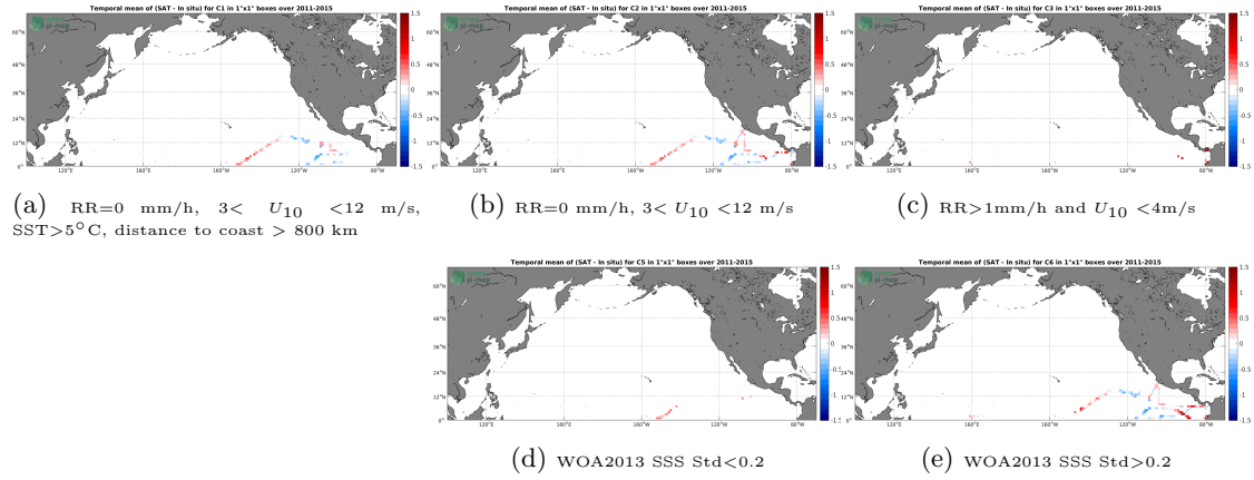
Figure 12: Temporal mean gridded over spatial boxes of size 1^\circ \times 1^\circ of \Delta SSS (SMOS L3 v2 - 9-Days (BEC) - TSG (GOSUD-Research-vessel)) for 5 different subdatasets corresponding to: RR=0 mm/h, 3 < U_{10} < 12 m/s, SST >5^\circ\text{C} , distance to coast > 800 km (a), RR=0 mm/h, 3 < U_{10} < 12 m/s (b), RR >1 mm/h and U_{10} < 4 m/s (c), WOA2013 SSS Std <0.2 (d), WOA2013 SSS Std >0.2 (e).
