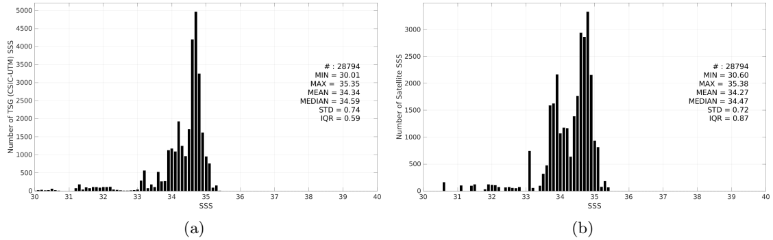
Figure 3: Histograms of SSS from TSG (CSIC-UTM) (a) and SMOS SSS L3 v2 - 9-Days (BEC) (b) considering all match-up pairs per bins of 0.1 over the North Pacific Ocean Pi-MEP region and for the full satellite product period.
