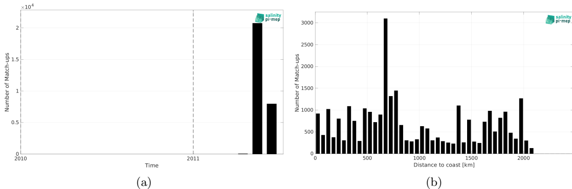
Figure 2: Number of match-ups between TSG (CSIC-UTM) and SMOS SSS L3 v2 - 9-Days (BEC) SSS as a function of time (a) and as function of the distance to coast (b) over the North Pacific Ocean Pi-MEP region and for the full satellite product period.
