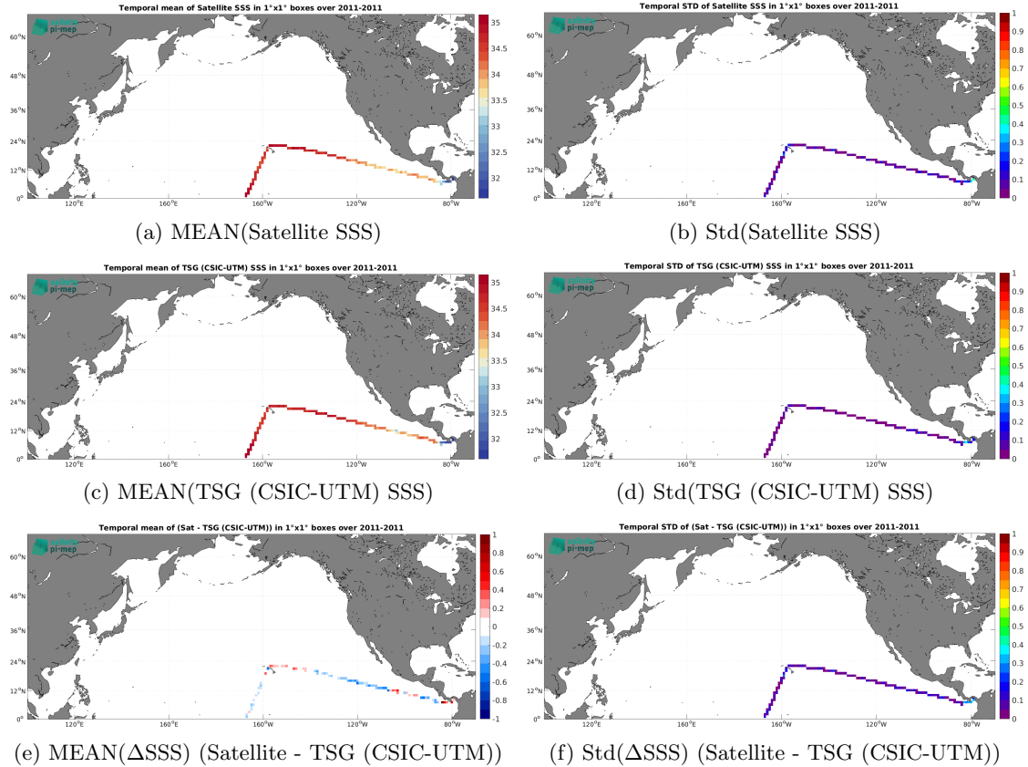
Figure 7: Temporal mean (left) and Std (right) of SSS from SMOS SSS L3 v2 - 9-Days (BEC) (top), TSG (CSIC-UTM) (middle), and of \Delta\text{SSS} (Satellite - TSG (CSIC-UTM)). Only match-up pairs are used to generate these maps.
