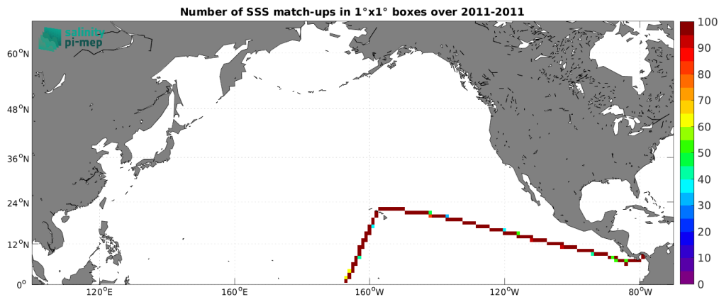
Figure 5: Number of SSS match-ups between TSG (CSIC-UTM) SSS and the SMOS SSS L3 v2 - 9-Days (BEC) SSS product for the North Pacific Ocean Pi-MEP region over 1^\circ \times 1^\circ boxes and for the full satellite product period.
