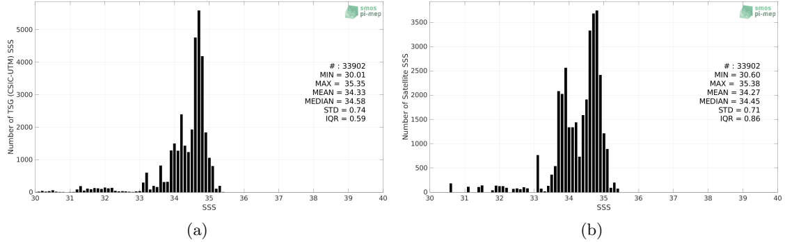
Figure 2: Histograms of SSS from TSG (CSIC-UTM) (a) and SMOS SSS L3 v2 - 9-Days (BEC) (b) considering all match-up pairs per bins of 0.1 over the North Pacific Ocean Pi-MEP region and for the full satellite product period.
