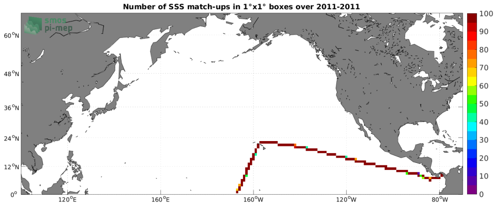
Figure 4: Number of SSS match-ups between TSG (CSIC-UTM) SSS and the SMOS SSS L3 v2 - 9-Days (BEC) SSS product for the North Pacific Ocean Pi-MEP region over 1^\circ \times 1^\circ boxes and for the full satellite product period.
