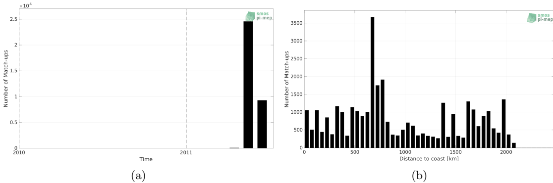
Figure 1: Number of match-ups between TSG (CSIC-UTM) and SMOS SSS L3 v2 - 9-Days (BEC) SSS as a function of time (a) and as function of the distance to coast (b) over the North Pacific Ocean Pi-MEP region and for the full satellite product period.
