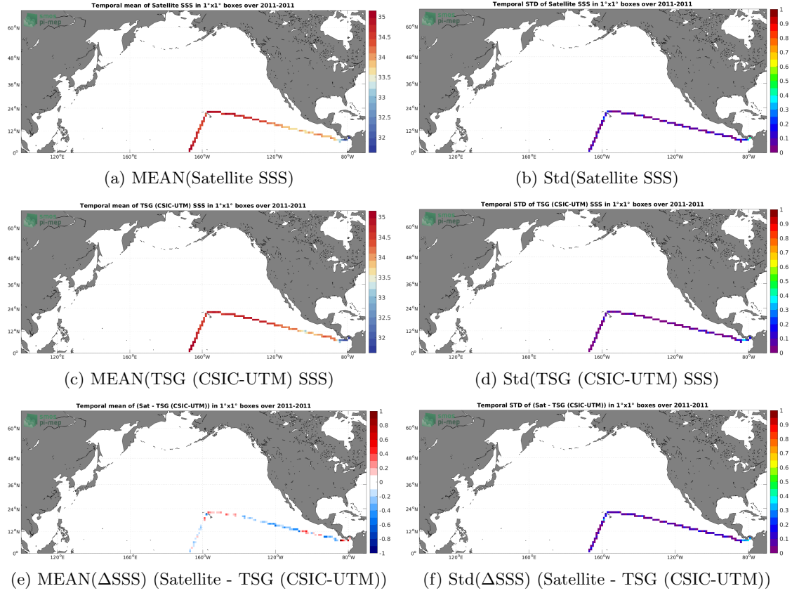
Figure 6: Temporal mean (left) and Std (right) of SSS from SMOS SSS L3 v2 - 9-Days (BEC) (top), TSG (CSIC-UTM) (middle), and of \Delta SSS (Satellite - TSG (CSIC-UTM)). Only match-up pairs are used to generate these maps.
