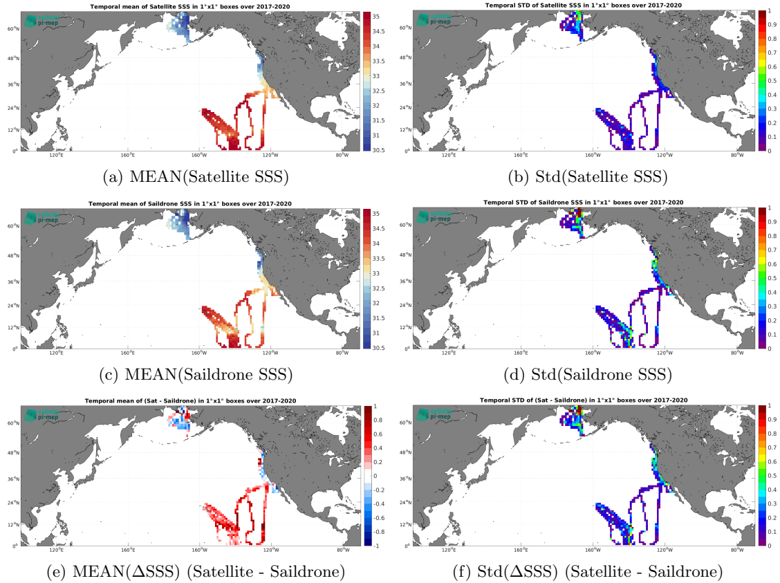
Figure 7: Temporal mean (left) and Std (right) of SSS from SMOS SSS L3 v2 - 9-Days (BEC) (top), Saildrone (middle), and of \Delta SSS (Satellite - Saildrone). Only match-up pairs are used to generate these maps.
