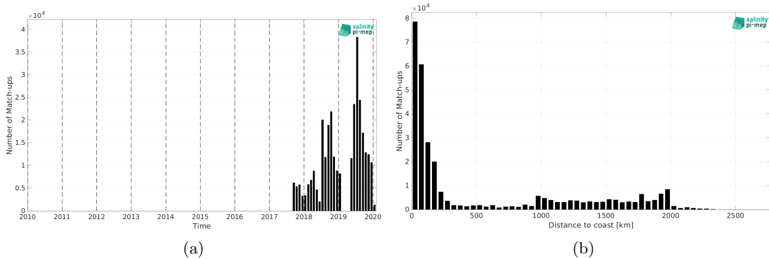
Figure 2: Number of match-ups between Saildrone and SMOS SSS L3 v2 - 9-Days (BEC) SSS as a function of time (a) and as function of the distance to coast (b) over the North Pacific Ocean Pi-MEP region and for the full satellite product period.
