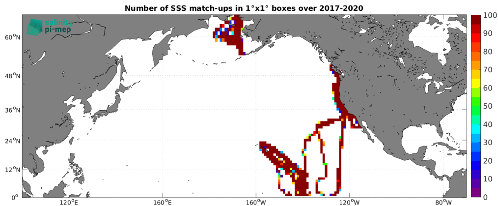
Figure 5: Number of SSS match-ups between Saildrone SSS and the SMOS SSS L3 v2 - 9-Days (BEC) SSS product for the North Pacific Ocean Pi-MEP region over 1^\circ \times 1^\circ boxes and for the full satellite product period.
