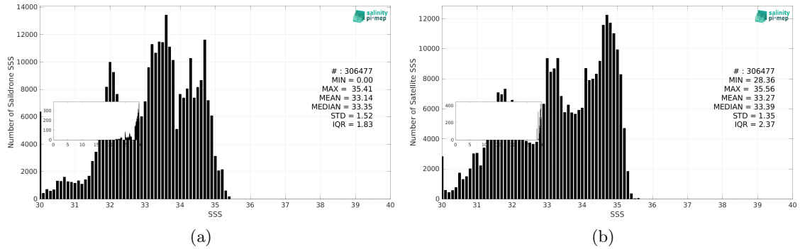
Figure 3: Histograms of SSS from Saildrone (a) and SMOS SSS L3 v2 - 9-Days (BEC) (b) considering all match-up pairs per bins of 0.1 over the North Pacific Ocean Pi-MEP region and for the full satellite product period.
