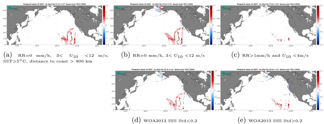
Figure 14: Temporal mean gridded over spatial boxes of size 1^\circ \times 1^\circ of \Delta SSS (SMOS SSS L3 v2 - 9-Days (BEC) - Saildrone) for 5 different subdatasets corresponding to:RR=0 mm/h, 3 < U_{10} < 12 m/s, SST >5^\circ\text{C} , distance to coast > 800 km (a), RR=0 mm/h, 3 < U_{10} < 12 m/s (b), RR >1 mm/h and U_{10} < 4 m/s (c), WOA2013 SSS Std <0.2 (d), WOA2013 SSS Std >0.2 (e).
