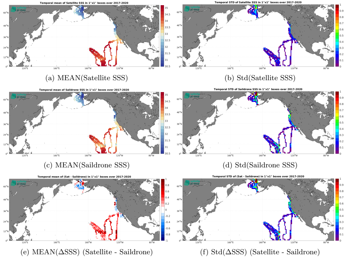
Figure 6: Temporal mean (left) and Std (right) of SSS from SMOS SSS L3 v2 - 9-Days (BEC) (top), Saildrone (middle), and of \Delta\text{SSS} (Satellite - Saildrone). Only match-up pairs are used to generate these maps.
