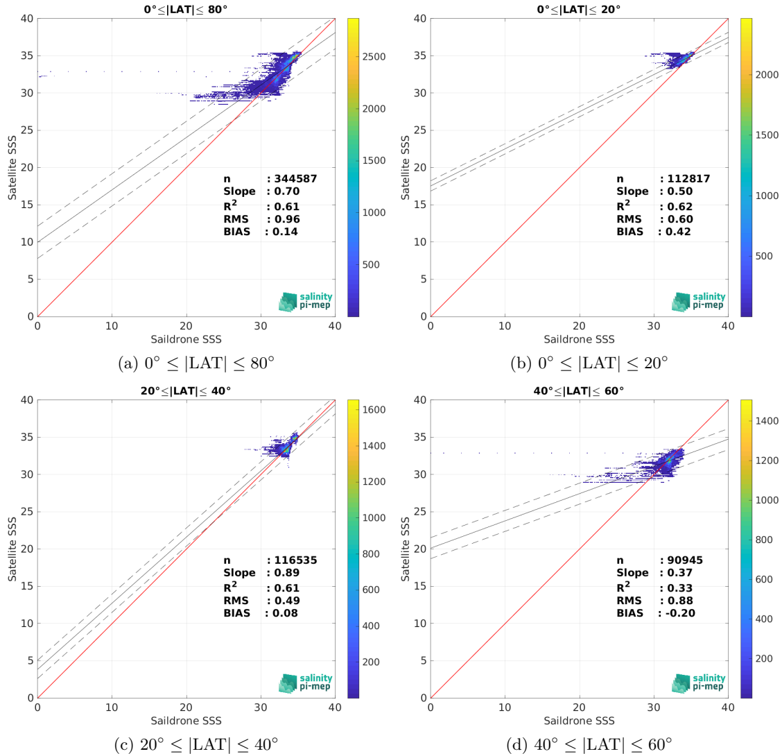
Figure 9: Contour maps of the concentration of SMOS SSS L3 v2 - 9-Days (BEC) SSS (y-axis) versus Sairdrone SSS (x-axis) at match-up pairs for different latitude bands. For each plot, the red line shows x=y . The black thin and dashed lines indicate a linear fit through the data cloud and the \pm 95\% confidence levels, respectively. The number match-up pairs n , the slope and R^2 coefficient of the linear fit, the root mean square (RMS) and the mean bias between satellite and in situ data are indicated for each latitude band in each plots.
