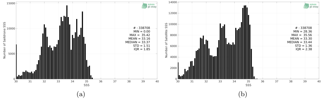
Figure 2: Histograms of SSS from Saildrone (a) and SMOS SSS L3 v2 - 9-Days (BEC) (b) considering all match-up pairs per bins of 0.1 over the North Pacific Ocean Pi-MEP region and for the full satellite product period.
