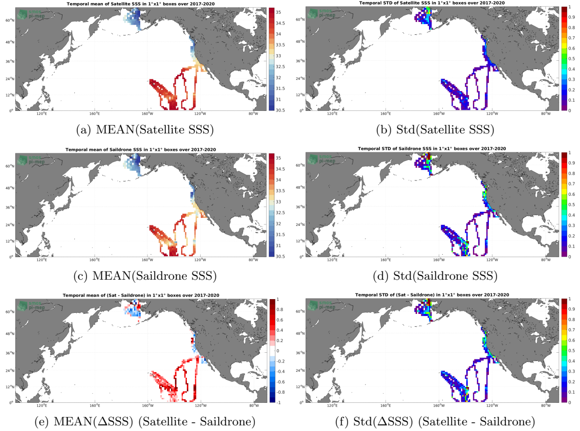
Figure 6: Temporal mean (left) and Std (right) of SSS from SMOS SSS L3 v2 - 9-Days (BEC) (top), Sairdrone (middle), and of \Delta SSS (Satellite - Sairdrone). Only match-up pairs are used to generate these maps.
