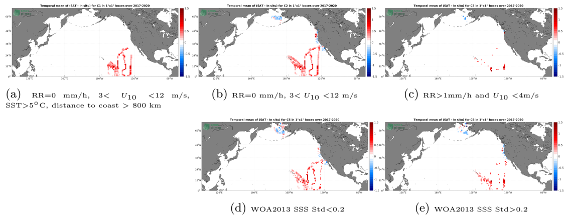
Figure 12: Temporal mean gridded over spatial boxes of size 1^\circ \times 1^\circ of \Delta SSS (SMOS SSS L3 v2 - 9-Days (BEC) - Saildrone) for 5 different subdatasets corresponding to:RR=0 mm/h, 3 < U_{10} < 12 m/s, SST >5^\circ\text{C} , distance to coast > 800 km (a), RR=0 mm/h, 3 < U_{10} < 12 m/s (b), RR >1 mm/h and U_{10} < 4 m/s (c), WOA2013 SSS Std <0.2 (d), WOA2013 SSS Std >0.2 (e).
