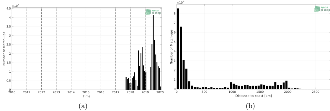
Figure 1: Number of match-ups between Saildrone and SMOS SSS L3 v2 - 9-Days (BEC) SSS as a function of time (a) and as function of the distance to coast (b) over the North Pacific Ocean Pi-MEP region and for the full satellite product period.
