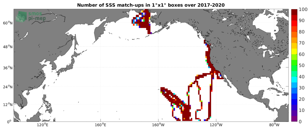
Figure 4: Number of SSS match-ups between Saildrone SSS and the SMOS SSS L3 v2 - 9-Days (BEC) SSS product for the North Pacific Ocean Pi-MEP region over 1^\circ \times 1^\circ boxes and for the full satellite product period.
