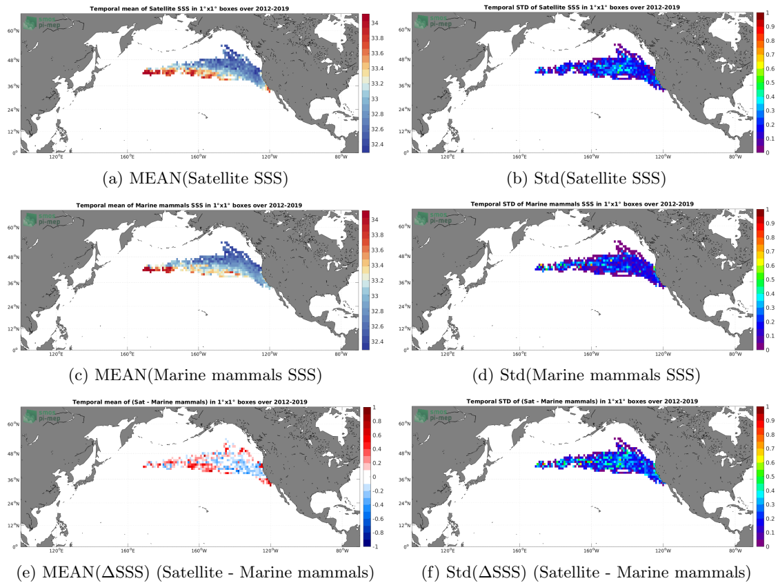
Figure 6: Temporal mean (left) and Std (right) of SSS from SMOS SSS L3 v2 - 9-Days (BEC) (top), Marine mammals (middle), and of \Delta SSS (Satellite - Marine mammals). Only match-up pairs are used to generate these maps.
