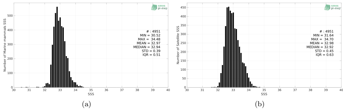
Figure 2: Histograms of SSS from Marine mammals (a) and SMOS SSS L3 v2 - 9-Days (BEC) (b) considering all match-up pairs per bins of 0.1 over the North Pacific Ocean Pi-MEP region and for the full satellite product period.
