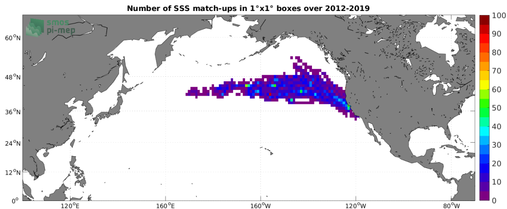
Figure 4: Number of SSS match-ups between Marine mammals SSS and the SMOS SSS L3 v2 - 9-Days (BEC) SSS product for the North Pacific Ocean Pi-MEP region over 1^\circ \times 1^\circ boxes and for the full satellite product period.
