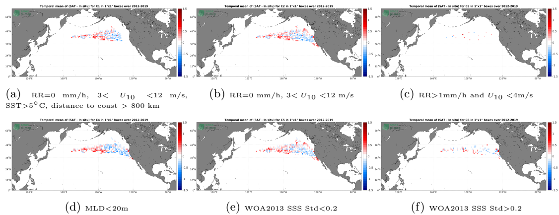
Figure 12: Temporal mean gridded over spatial boxes of size 1^\circ \times 1^\circ of \Delta SSS (SMOS SSS L3 v2 - 9-Days (BEC) - Marine mammals) for 6 different subdatasets corresponding to:RR=0 mm/h, 3 < U_{10} < 12 m/s, SST >5^\circ\text{C} , distance to coast > 800 km (a), RR=0 mm/h, 3 < U_{10} < 12 m/s (b), RR >1 mm/h and U_{10} < 4 m/s (c),MLD <20 m (d),WOA2013 SSS Std <0.2 (e),WOA2013 SSS Std >0.2 (f).
