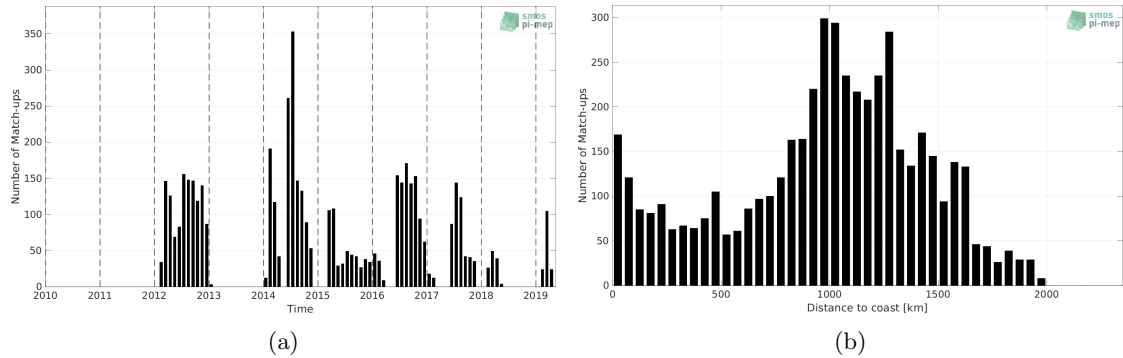
Figure 1: Number of match-ups between Marine mammals and SMOS SSS L3 v2 - 9-Days (BEC) SSS as a function of time (a) and as function of the distance to coast (b) over the North Pacific Ocean Pi-MEP region and for the full satellite product period.
