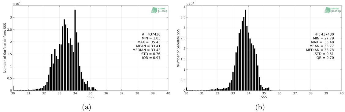
Figure 2: Histograms of SSS from Surface drifters (a) and SMOS SSS L3 v2 - 9-Days (BEC) (b) considering all match-up pairs per bins of 0.1 over the North Pacific Ocean Pi-MEP region and for the full satellite product period.
