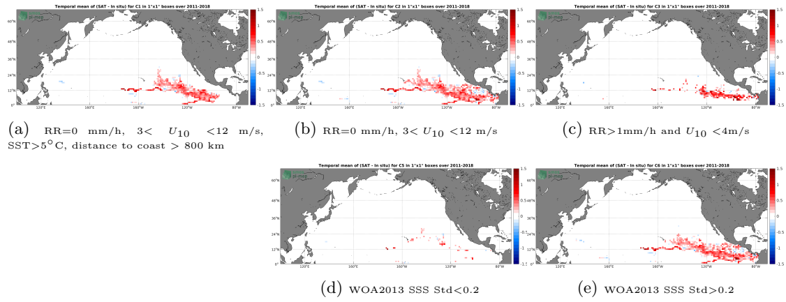
Figure 11: Temporal mean gridded over spatial boxes of size 1^\circ \times 1^\circ of \Delta SSS (SMOS SSS L3 v2 - 9-Days (BEC) - Surface drifters) for 5 different subdatasets corresponding to: RR=0 mm/h, 3 < U_{10} < 12 m/s, SST >5^\circ\text{C} , distance to coast > 800 km (a), RR=0 mm/h, 3 < U_{10} < 12 m/s (b), RR >1 mm/h and U_{10} < 4 m/s (c), WOA2013 SSS Std <0.2 (d), WOA2013 SSS Std >0.2 (e).
