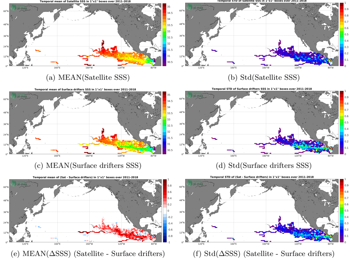
Figure 5: Temporal mean (left) and Std (right) of SSS from SMOS SSS L3 v2 - 9-Days (BEC) (top), Surface drifters (middle), and of \Delta SSS (Satellite - Surface drifters). Only match-up pairs are used to generate these maps.
