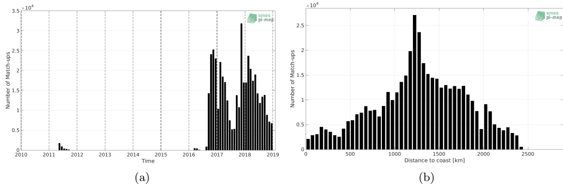
Figure 1: Number of match-ups between Surface drifters and SMOS SSS L3 v2 - 9-Days (BEC) SSS as a function of time (a) and as function of the distance to coast (b) over the North Pacific Ocean Pi-MEP region and for the full satellite product period.
