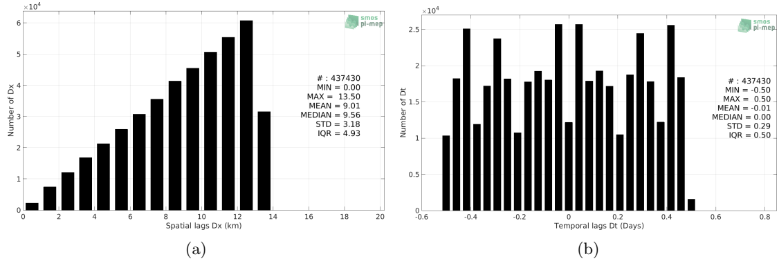
Figure 4: Histograms of the spatial (a) and temporal (b) lags between the time of the Surface drifters measurements and the date of the corresponding SMOS SSS L3 v2 - 9-Days (BEC) SSS product.
