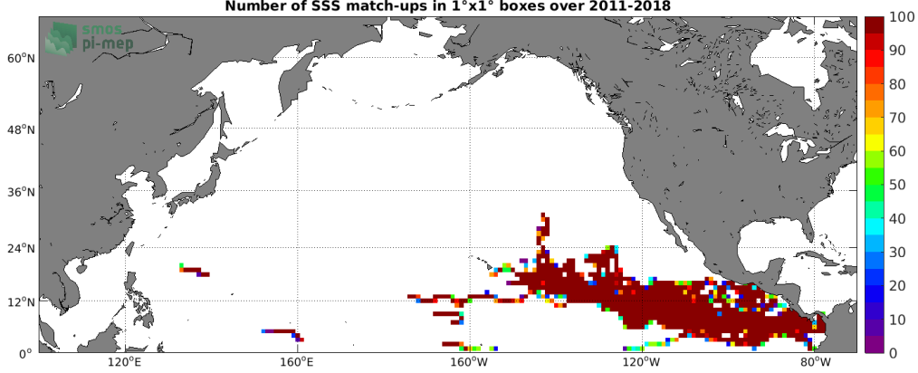
Figure 3: Number of SSS match-ups between Surface drifters SSS and the SMOS SSS L3 v2 - 9-Days (BEC) SSS product for the North Pacific Ocean Pi-MEP region over 1^\circ \times 1^\circ boxes and for the full satellite product period.
