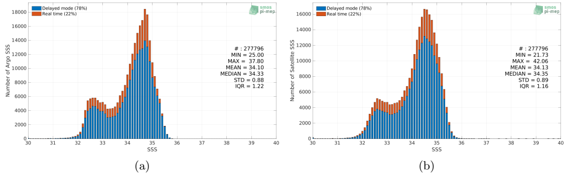
Figure 2: Histograms of SSS from Argo (a) and SMOS SSS L3 v2 - 9-Days (BEC) (b) considering all match-up pairs per bins of 0.1 over the North Pacific Ocean Pi-MEP region and for the full satellite product period.
