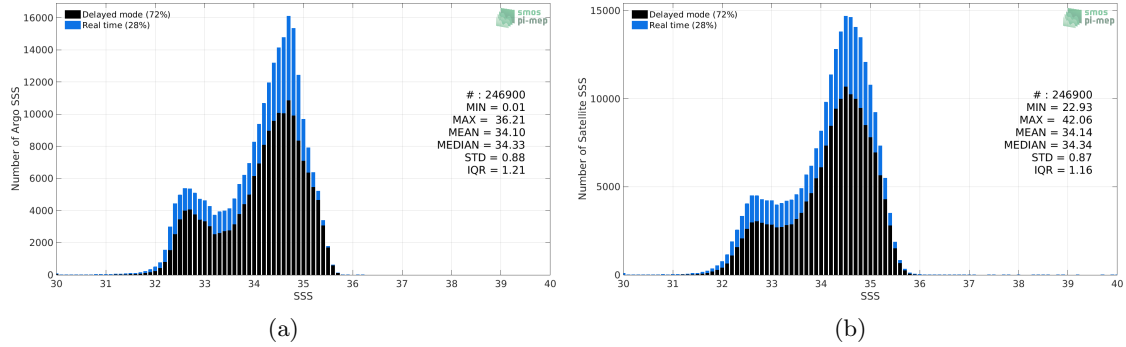
Figure 2: Histograms of SSS from Argo (a) and SMOS SSS L3 v2 - 9-Days (BEC) (b) considering all match-up pairs per bins of 0.1 over the North Pacific Ocean Pi-MEP region and for the full satellite product period.
