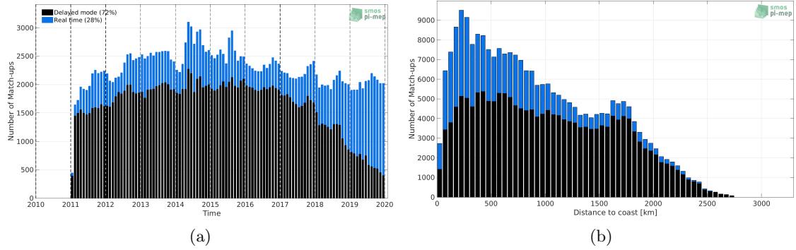
Figure 1: Number of match-ups between Argo and SMOS SSS L3 v2 - 9-Days (BEC) SSS as a function of time (a) and as function of the distance to coast (b) over the North Pacific Ocean Pi-MEP region and for the full satellite product period.
