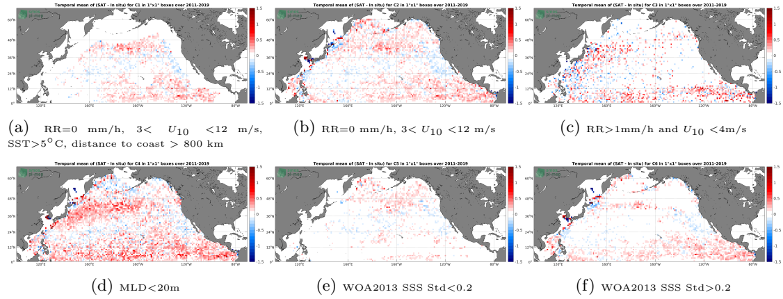
Figure 12: Temporal mean gridded over spatial boxes of size 1^\circ \times 1^\circ of \Delta SSS (SMOS SSS L3 v2 - 9-Days (BEC) - Argo) for 6 different subdatasets corresponding to: RR=0 mm/h, 3 < U_{10} < 12 m/s, SST > 5^\circ C , distance to coast > 800 km (a), RR=0 mm/h, 3 < U_{10} < 12 m/s (b), RR > 1 mm/h and U_{10} < 4 m/s (c), MLD < 20 m (d), WOA2013 SSS Std < 0.2 (e), WOA2013 SSS Std > 0.2 (f).
