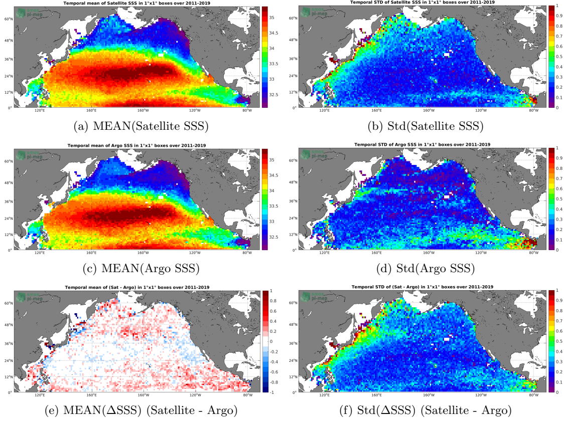
Figure 6: Temporal mean (left) and Std (right) of SSS from SMOS SSS L3 v2 - 9-Days (BEC) (top), Argo (middle), and of \Delta SSS (Satellite - Argo). Only match-up pairs are used to generate these maps.
