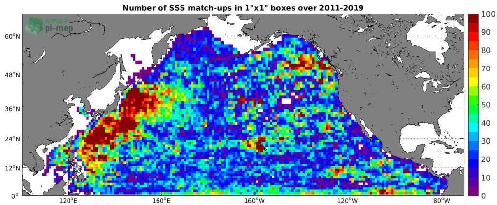
Figure 4: Number of SSS match-ups between Argo SSS and the SMOS SSS L3 v2 - 9-Days (BEC) SSS product for the North Pacific Ocean Pi-MEP region over 1^\circ \times 1^\circ boxes and for the full satellite product period.
