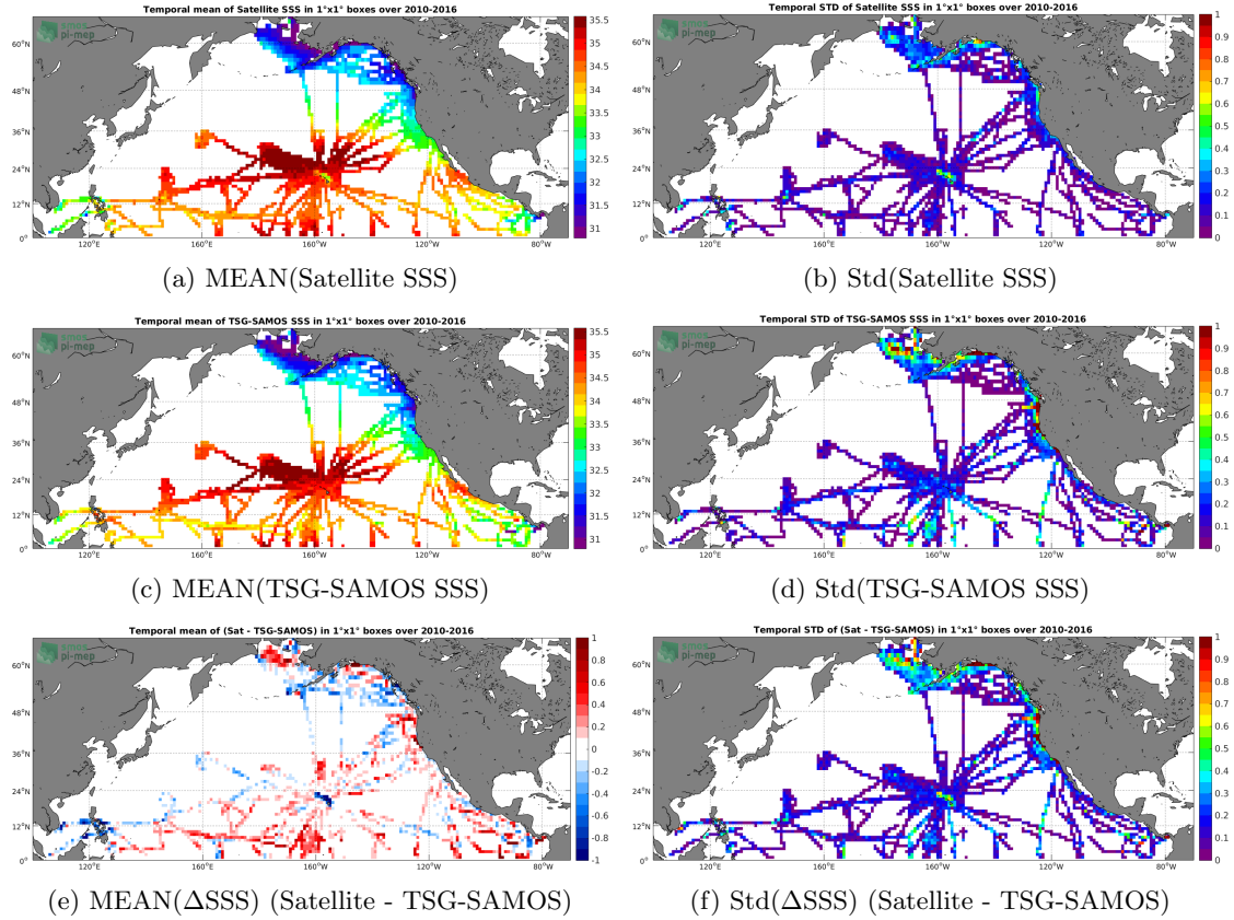
Figure 6: Temporal mean (left) and Std (right) of SSS from SMOS-L3-BEC-OA-V1-9DAYS-0.25DEG (top), TSG-SAMOS (middle), and of \Delta SSS (Satellite - TSG-SAMOS). Only match-up pairs are used to generate these maps.
