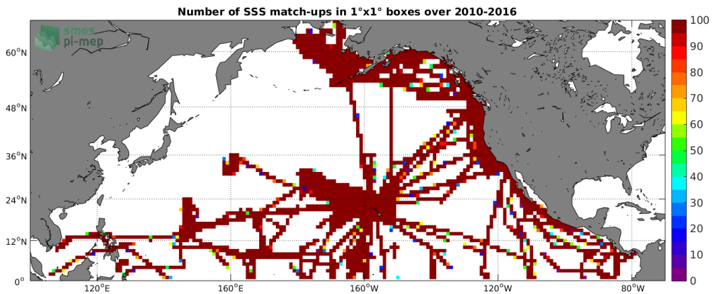
Figure 4: Number of SSS match-ups between TSG-SAMOS SSS and the SMOS-L3-BEC-OA-V1-9DAYS-0.25DEG SSS product for the North Pacific Ocean Pi-MEP region over 1^\circ \times 1^\circ boxes and for the full satellite product period.
