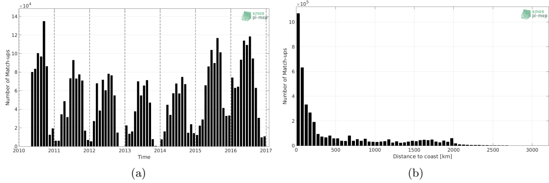
Figure 1: Number of match-ups between TSG-SAMOS and SMOS-L3-BEC-OA-V1-9DAYS-0.25DEG SSS as a function of time (a) and as function of the distance to coast (b) over the North Pacific Ocean Pi-MEP region and for the full satellite product period.
