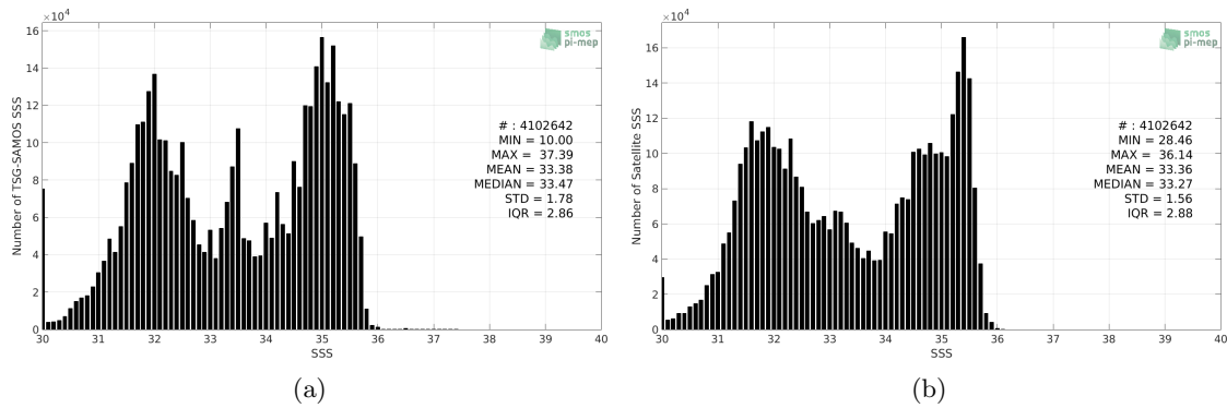
Figure 2: Histograms of SSS from TSG-SAMOS (a) and SMOS-L3-BEC-OA-V1-9DAYS-0.25DEG (b) considering all match-up pairs per bins of 0.1 over the North Pacific Ocean Pi-MEP region and for the full satellite product period.
