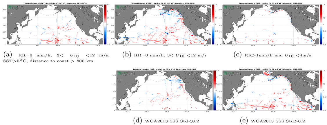
Figure 12: Temporal mean gridded over spatial boxes of size 1^\circ \times 1^\circ of \Delta SSS (SMOS-L3-BEC-OA-V1-9DAYS-0.25DEG - TSG-SAMOS) for 5 different subdatasets corresponding to:RR=0 mm/h, 3 < U_{10} < 12 m/s, SST > 5^\circ C , distance to coast > 800 km (a), RR=0 mm/h, 3 < U_{10} < 12 m/s (b), RR>1mm/h and U_{10} < 4 m/s (c), WOA2013 SSS Std<0.2 (d), WOA2013 SSS Std>0.2 (e).
