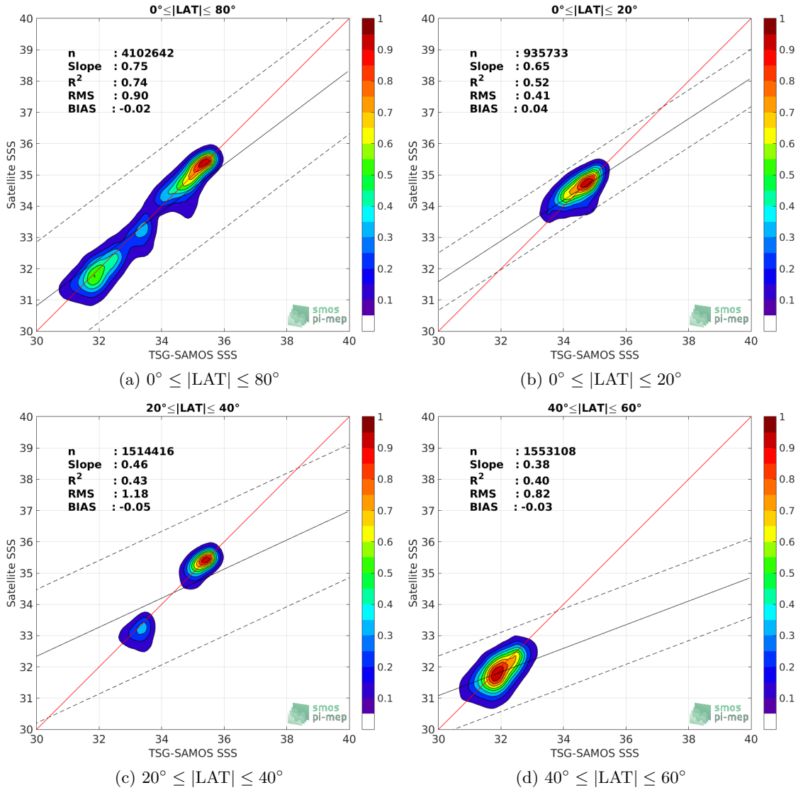
Figure 9: Contour maps of the concentration of SMOS-L3-BEC-OA-V1-9DAYS-0.25DEG SSS (y-axis) versus TSG-SAMOS SSS (x-axis) at match-up pairs for different latitudinal bands. For each plot, the red line shows x=y . The black thin and dashed lines indicate a linear fit through the data cloud and the \pm 95\% confidence levels, respectively. The number match-up pairs n , the slope and R^2 coefficient of the linear fit, the root mean square (RMS) and the mean bias between satellite and in situ data are indicated for each latitude band in each plots.
