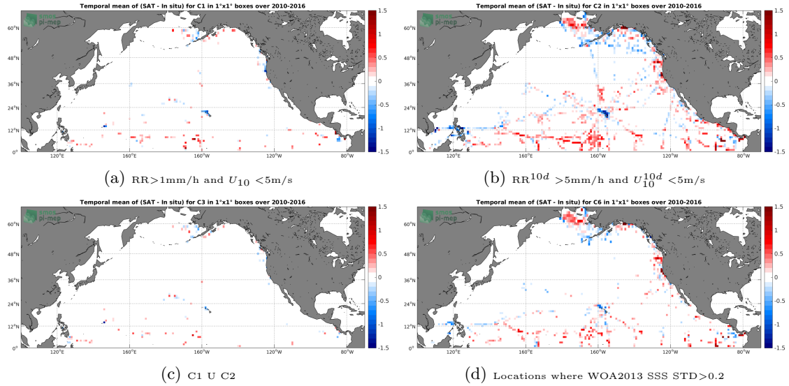
Figure 12: Temporal mean gridded over spatial boxes of size 1^\circ \times 1^\circ of \Delta SSS (SMOS-L3-BEC-OA-V1-9DAYS-0.25DEG - TSG-SAMOS) for 4 different subdatasets corresponding to: RR > 1\text{mm/h} and U_{10} < 5\text{m/s} (a), RR^{10d} > 5\text{mm/h} and U_{10}^{10d} < 5\text{m/s} (b), C1 U C2 (c), Locations where WOA2013 SSS STD > 0.2 (d).
