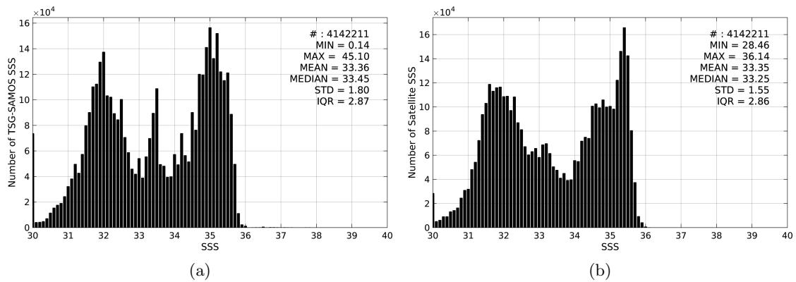
Figure 2: Histograms of SSS from TSG-SAMOS (a) and SMOS-L3-BEC-OA-V1-9DAYS-0.25DEG (b) considering all match-up pairs per bins of 0.1 over the North Pacific Ocean Pi-MEP region and for the full satellite product period.
