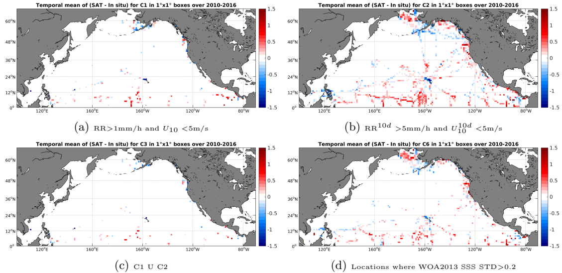
Figure 12: Temporal mean gridded over spatial boxes of size 1^\circ \times 1^\circ of \Delta SSS (SMOS-L3-BEC-OA-V1-9DAYS-0.25DEG - TSG-SAMOS) for 4 different subdatasets corresponding to:RR>1mm/h and U_{10} < 5\text{m/s} (a), RR^{10d} > 5\text{mm/h} and U_{10}^{10d} < 5\text{m/s} (b), C1 U C2 (c),Locations where WOA2013 SSS STD>0.2 (d).
