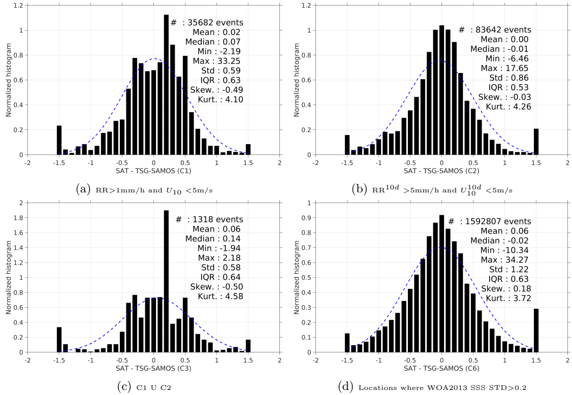
Figure 13: Normalized histogram of \Delta SSS (SMOS-L3-BEC-OA-V1-9DAYS-0.25DEG - TSG-SAMOS) for 6 different subdatasets corresponding to: RR > 1\text{mm/h} and U_{10} < 5\text{m/s} (a), RR^{10d} > 5\text{mm/h} and U_{10}^{10d} < 5\text{m/s} (b), C1 U C2 (c), Locations where WOA2013 SSS STD > 0.2 (d).
