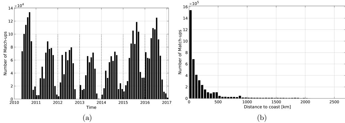
Figure 1: Number of match-ups between TSG-SAMOS and SMOS-L3-BEC-OA-V1-9DAYS-0.25DEG SSS as a function of time (a) and as function of the distance to coast (b) over the North Pacific Ocean Pi-MEP region and for the full satellite product period.
