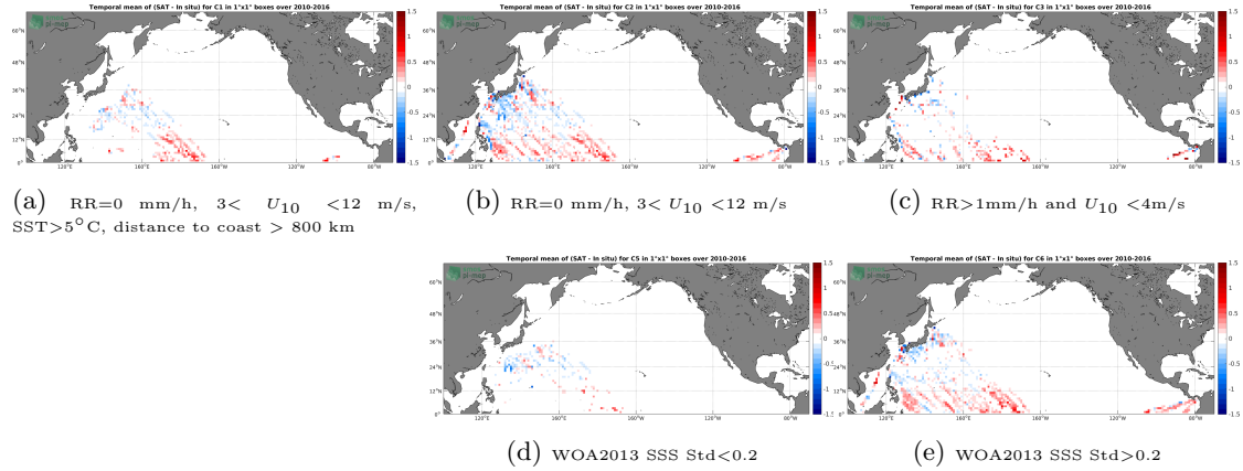
Figure 12: Temporal mean gridded over spatial boxes of size 1^\circ \times 1^\circ of \Delta SSS (SMOS-L3-BEC-OA-V1-9DAYS-0.25DEG - TSG-LEGOS-DM) for 5 different subdatasets corresponding to: RR=0 mm/h, 3 < U_{10} < 12 m/s, SST > 5^\circ\text{C} , distance to coast > 800 km (a), RR=0 mm/h, 3 < U_{10} < 12 m/s (b), RR > 1 mm/h and U_{10} < 4 m/s (c), WOA2013 SSS Std < 0.2 (d), WOA2013 SSS Std > 0.2 (e).
