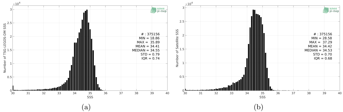
Figure 2: Histograms of SSS from TSG-LEGOS-DM (a) and SMOS-L3-BEC-OA-V1-9DAYS-0.25DEG (b) considering all match-up pairs per bins of 0.1 over the North Pacific Ocean Pi-MEP region and for the full satellite product period.
