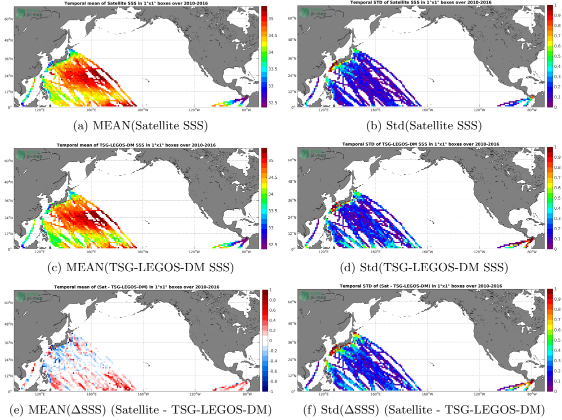
Figure 6: Temporal mean (left) and Std (right) of SSS from SMOS-L3-BEC-OA-V1-9DAYS-0.25DEG (top), TSG-LEGOS-DM (middle), and of \Delta SSS (Satellite - TSG-LEGOS-DM). Only match-up pairs are used to generate these maps.
