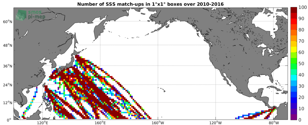
Figure 4: Number of SSS match-ups between TSG-LEGOS-DM SSS and the SMOS-L3-BEC-OA-V1-9DAYS-0.25DEG SSS product for the North Pacific Ocean Pi-MEP region over 1°x1° boxes and for the full satellite product period.
