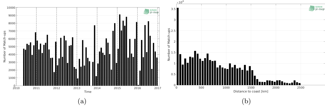
Figure 1: Number of match-ups between TSG-LEGOS-DM and SMOS-L3-BEC-OA-V1-9DAYS-0.25DEG SSS as a function of time (a) and as function of the distance to coast (b) over the North Pacific Ocean Pi-MEP region and for the full satellite product period.
