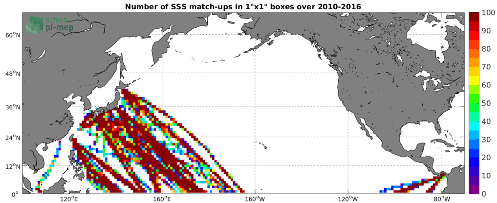
Figure 4: Number of SSS match-ups between TSG-LEGOS-DM SSS and the SMOS-L3-BEC-OA-V1-9DAYS-0.25DEG SSS product for the North Pacific Ocean Pi-MEP region over 1^\circ \times 1^\circ boxes and for the full satellite product period.
