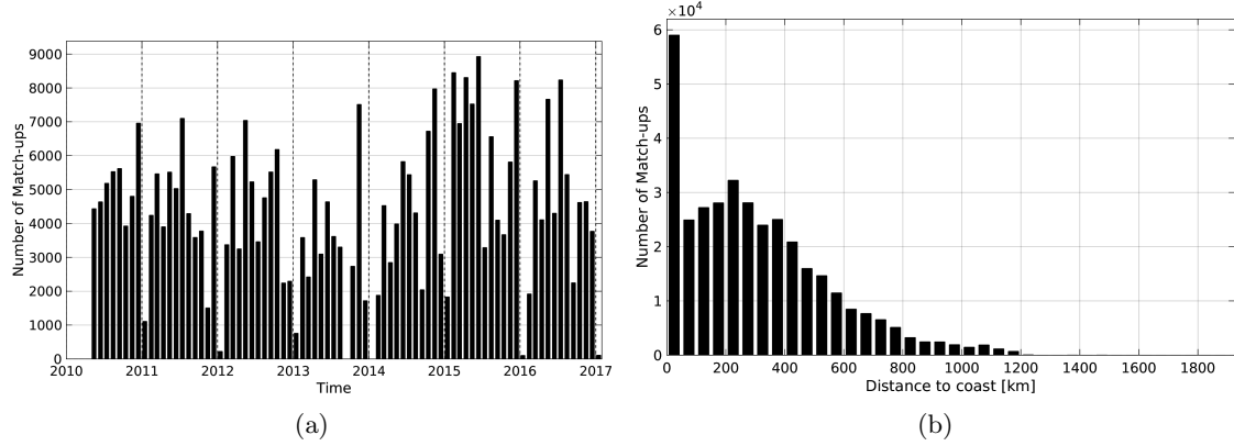
Figure 1: Number of match-ups between TSG-LEGOS-DM and SMOS-L3-BEC-OA-V1-9DAYS-0.25DEG SSS as a function of time (a) and as function of the distance to coast (b) over the North Pacific Ocean Pi-MEP region and for the full satellite product period.
