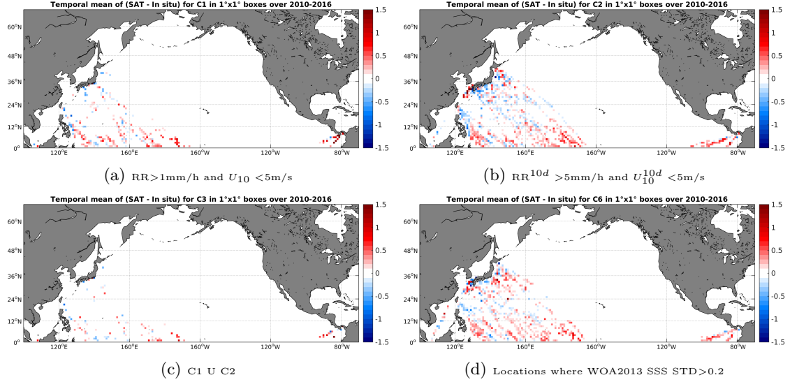
Figure 12: Temporal mean gridded over spatial boxes of size 1^\circ \times 1^\circ of \Delta SSS (SMOS-L3-BEC-OA-V1-9DAYS-0.25DEG - TSG-LEGOS-DM) for 4 different subdatasets corresponding to: RR > 1 mm/h and U_{10} < 5 m/s (a), RR^{10d} > 5 mm/h and U_{10}^{10d} < 5 m/s (b), C1 U C2 (c), Locations where WOA2013 SSS STD > 0.2 (d).
