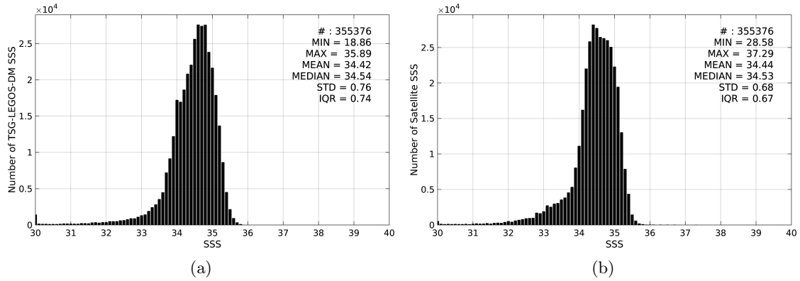
Figure 2: Histograms of SSS from TSG-LEGOS-DM (a) and SMOS-L3-BEC-OA-V1-9DAYS-0.25DEG (b) considering all match-up pairs per bins of 0.1 over the North Pacific Ocean Pi-MEP region and for the full satellite product period.
