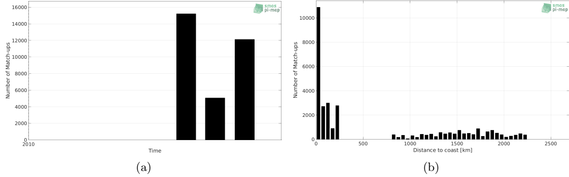
Figure 1: Number of match-ups between TSG-GOSUD-Sailing-ship and SMOS-L3-BEC-OA-V1-9DAYS-0.25DEG SSS as a function of time (a) and as function of the distance to coast (b) over the North Pacific Ocean Pi-MEP region and for the full satellite product period.
