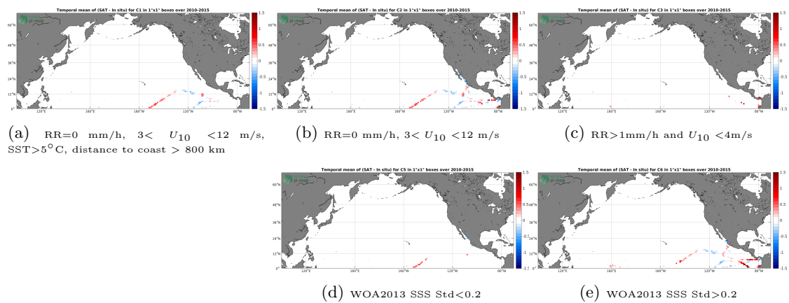
Figure 12: Temporal mean gridded over spatial boxes of size 1^\circ \times 1^\circ of \Delta SSS (SMOS-L3-BEC-OA-V1-9DAYS-0.25DEG - TSG-GOSUD-Research-vessel) for 5 different subdatasets corresponding to:RR=0 mm/h, 3 < U_{10} < 12 m/s, SST >5^\circ\text{C} , distance to coast > 800 km (a), RR=0 mm/h, 3 < U_{10} < 12 m/s (b), RR >1 mm/h and U_{10} < 4 m/s (c), WOA2013 SSS Std <0.2 (d), WOA2013 SSS Std >0.2 (e).
