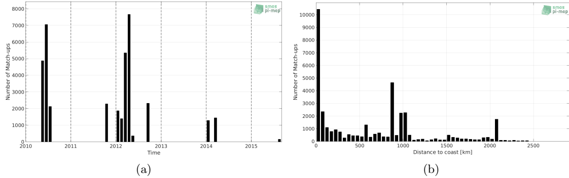
Figure 1: Number of match-ups between TSG-GOSUD-Research-vessel and SMOS-L3-BEC-OA-V1-9DAYS-0.25DEG SSS as a function of time (a) and as function of the distance to coast (b) over the North Pacific Ocean Pi-MEP region and for the full satellite product period.
