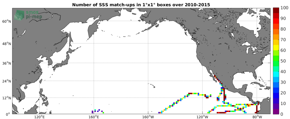
Figure 4: Number of SSS match-ups between TSG-GOSUD-Research-vessel SSS and the SMOS-L3-BEC-OA-V1-9DAYS-0.25DEG SSS product for the North Pacific Ocean Pi-MEP region over 1°x1° boxes and for the full satellite product period.
