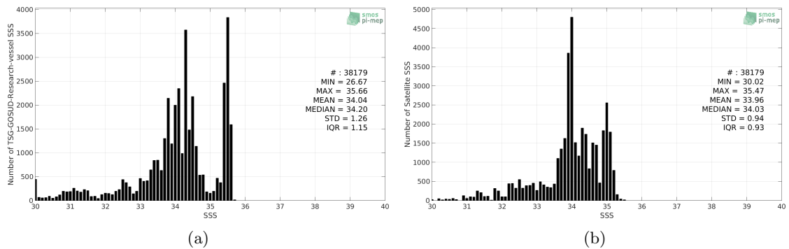
Figure 2: Histograms of SSS from TSG-GOSUD-Research-vessel (a) and SMOS-L3-BEC-OA-V1-9DAYS-0.25DEG (b) considering all match-up pairs per bins of 0.1 over the North Pacific Ocean Pi-MEP region and for the full satellite product period.
