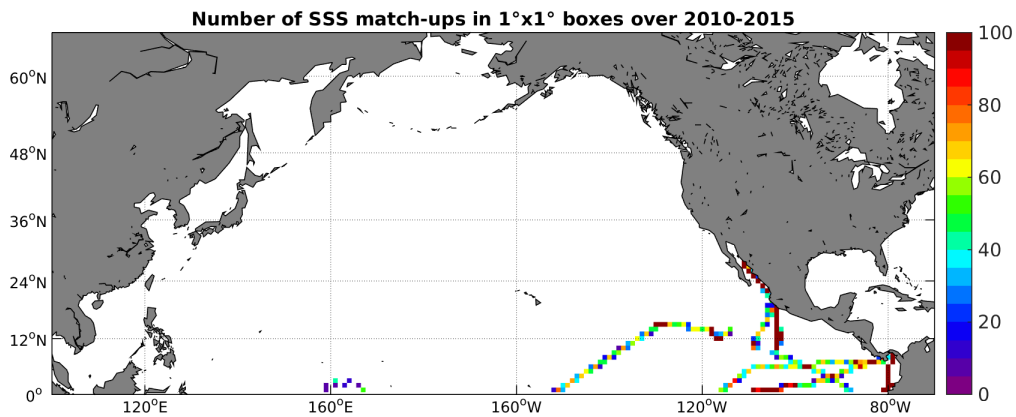
Figure 4: Number of SSS match-ups between TSG-GOSUD-Research-vessel SSS and the SMOS-L3-BEC-OA-V1-9DAYS-0.25DEG SSS product for the North Pacific Ocean Pi-MEP region over 1^\circ \times 1^\circ boxes and for the full satellite product period.
