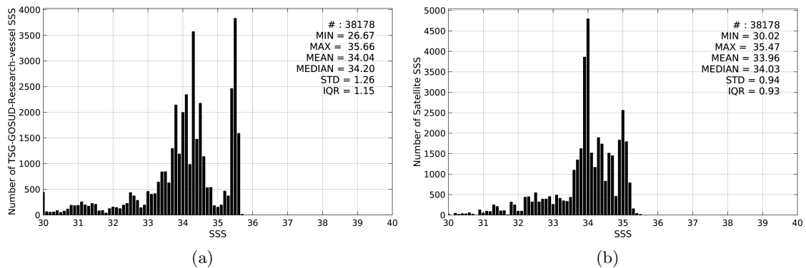
Figure 2: Histograms of SSS from TSG-GOSUD-Research-vessel (a) and SMOS-L3-BEC-OA-V1-9DAYS-0.25DEG (b) considering all match-up pairs per bins of 0.1 over the North Pacific Ocean Pi-MEP region and for the full satellite product period.
