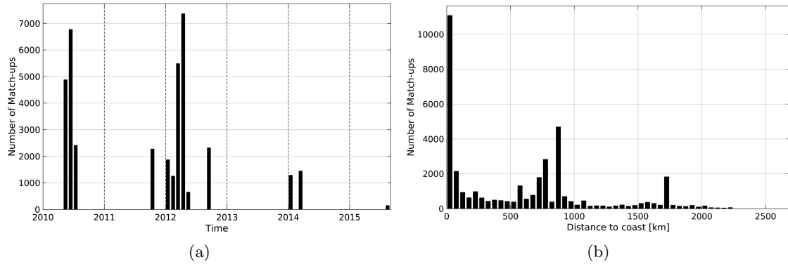
Figure 1: Number of match-ups between TSG-GOSUD-Research-vessel and SMOS-L3-BEC-OA-V1-9DAYS-0.25DEG SSS as a function of time (a) and as function of the distance to coast (b) over the North Pacific Ocean Pi-MEP region and for the full satellite product period.
