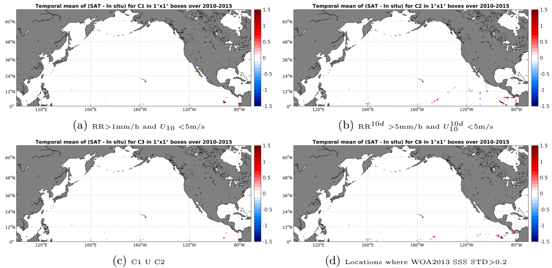
Figure 12: Temporal mean gridded over spatial boxes of size 1^\circ \times 1^\circ of \Delta SSS (SMOS-L3-BEC-OA-V1-9DAYS-0.25DEG - TSG-GOSUD-Research-vessel) for 4 different subdatasets corresponding to: RR > 1\text{mm/h} and U_{10} < 5\text{m/s} (a), RR^{10d} > 5\text{mm/h} and U_{10}^{10d} < 5\text{m/s} (b), C1 U C2 (c), Locations where WOA2013 SSS STD > 0.2 (d).
