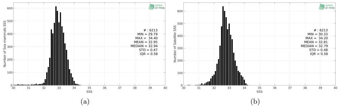
Figure 2: Histograms of SSS from Sea mammals (a) and SMOS-L3-BEC-OA-V1-9DAYS-0.25DEG (b) considering all match-up pairs per bins of 0.1 over the North Pacific Ocean Pi-MEP region and for the full satellite product period.
