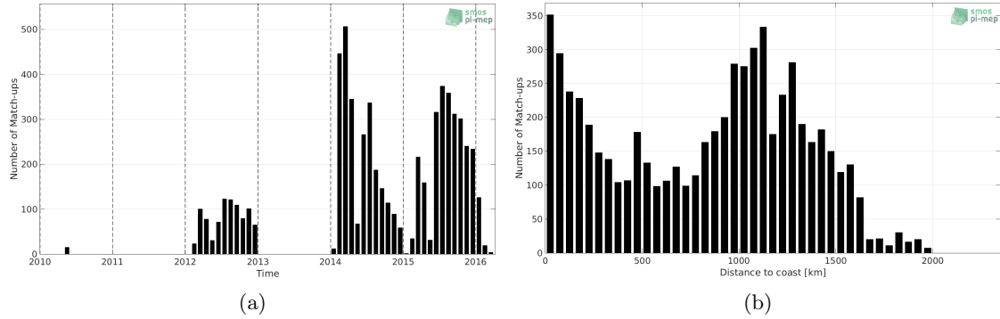
Figure 1: Number of match-ups between Sea mammals and SMOS-L3-BEC-OA-V1-9DAYS-0.25DEG SSS as a function of time (a) and as function of the distance to coast (b) over the North Pacific Ocean Pi-MEP region and for the full satellite product period.
