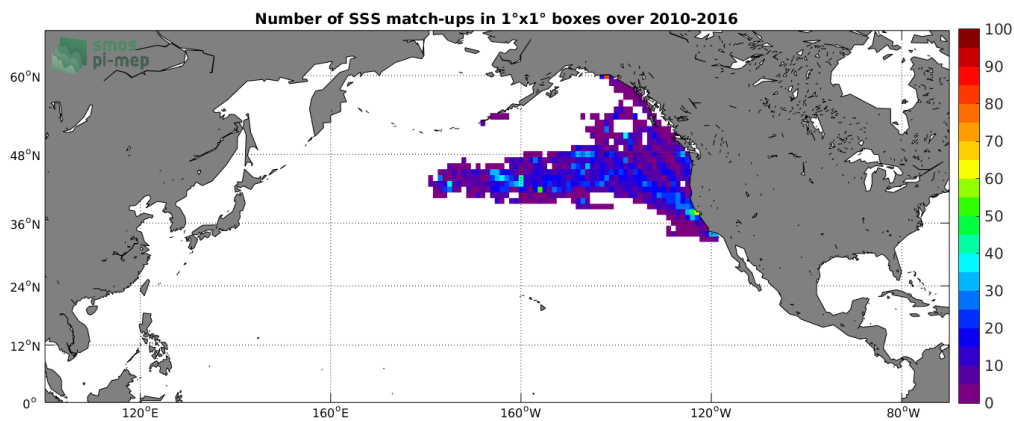
Figure 4: Number of SSS match-ups between Sea mammals SSS and the SMOS-L3-BEC-OA-V1-9DAYS-0.25DEG SSS product for the North Pacific Ocean Pi-MEP region over 1°x1° boxes and for the full satellite product period.
