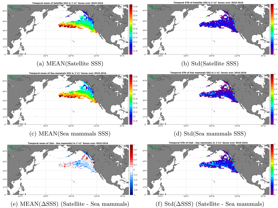
Figure 6: Temporal mean (left) and Std (right) of SSS from SMOS-L3-BEC-OA-V1-9DAYS-0.25DEG (top), Sea mammals (middle), and of \Delta SSS (Satellite - Sea mammals). Only match-up pairs are used to generate these maps.
