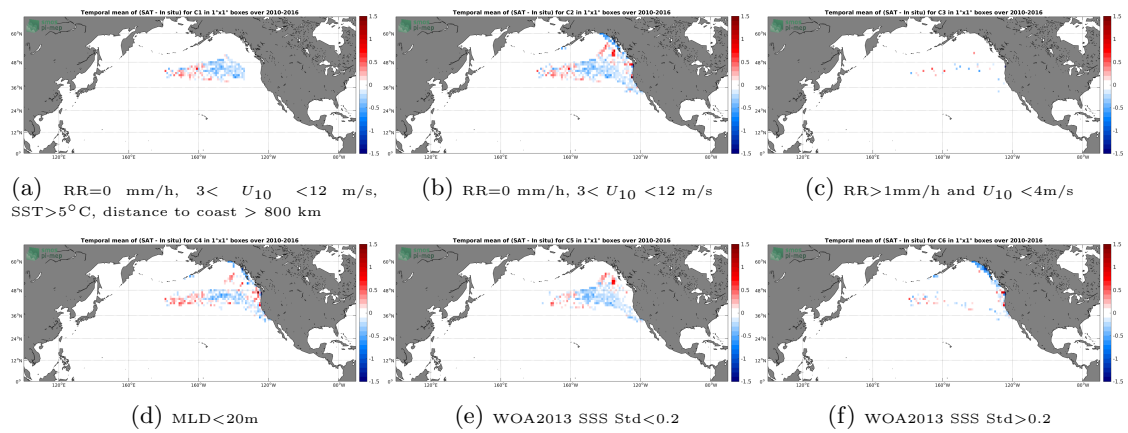
Figure 12: Temporal mean gridded over spatial boxes of size 1^\circ \times 1^\circ of \Delta SSS (SMOS-L3-BEC-OA-V1-9DAYS-0.25DEG - Sea mammals) for 6 different subdatasets corresponding to:RR=0 mm/h, 3 < U_{10} < 12 m/s, SST >5^\circ C, distance to coast > 800 km (a), RR=0 mm/h, 3 < U_{10} < 12 m/s (b), RR >1 mm/h and U_{10} < 4 m/s (c),MLD <20 m (d),WOA2013 SSS Std <0.2 (e),WOA2013 SSS Std >0.2 (f).
