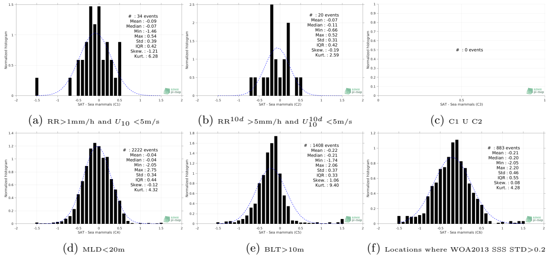
Figure 13: Normalized histogram of ΔSSS (SMOS-L3-BEC-OA-V1-9DAYS-0.25DEG - Sea mammals) for 6 different subdatasets corresponding to: RR>1mm/h and U_{10} < 5\text{m/s} (a), RR^{10d} > 5\text{mm/h} and U_{10}^{10d} < 5\text{m/s} (b), C1 U C2 (c),MLD<20m (d),BLT>10m (e),Locations where WOA2013 SSS STD>0.2 (f).
