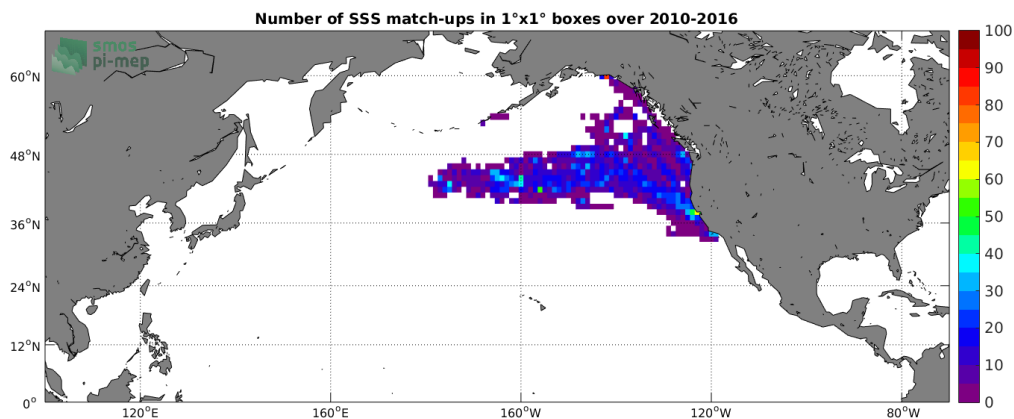
Figure 4: Number of SSS match-ups between Sea mammals SSS and the SMOS-L3-BEC-OA-V1-9DAYS-0.25DEG SSS product for the North Pacific Ocean Pi-MEP region over 1^\circ \times 1^\circ boxes and for the full satellite product period.
