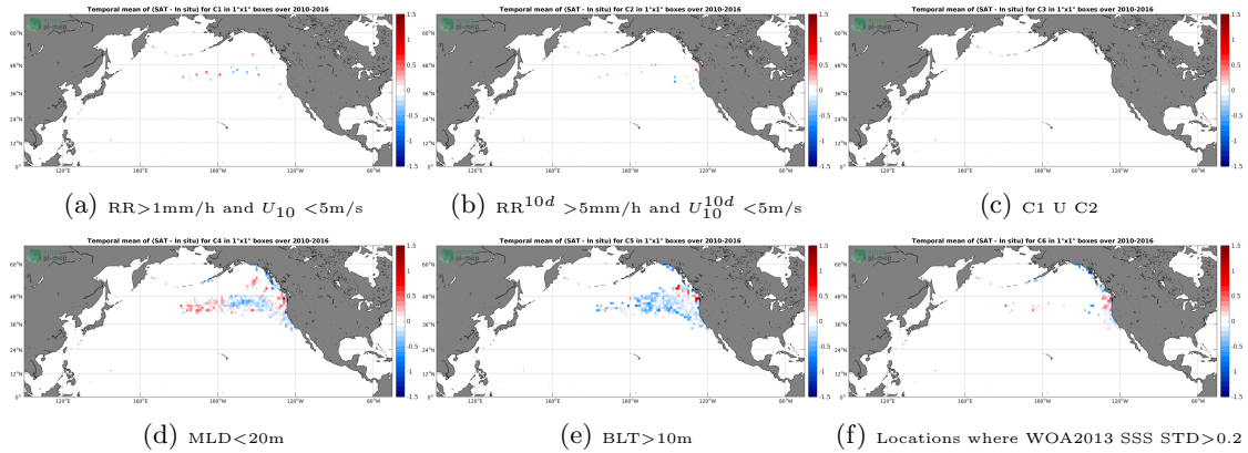
Figure 12: Temporal mean gridded over spatial boxes of size 1°x1° of ΔSSS (SMOS-L3-BEC-OA-V1-9DAYS-0.25DEG - Sea mammals) for 6 different subdatasets corresponding to:RR>1mm/h and U_{10} < 5\text{m/s} (a), RR^{10d} > 5\text{mm/h} and U_{10}^{10d} < 5\text{m/s} (b), C1 U C2 (c),MLD<20m (d),BLT>10m (e),Locations where WOA2013 SSS STD>0.2 (f).
